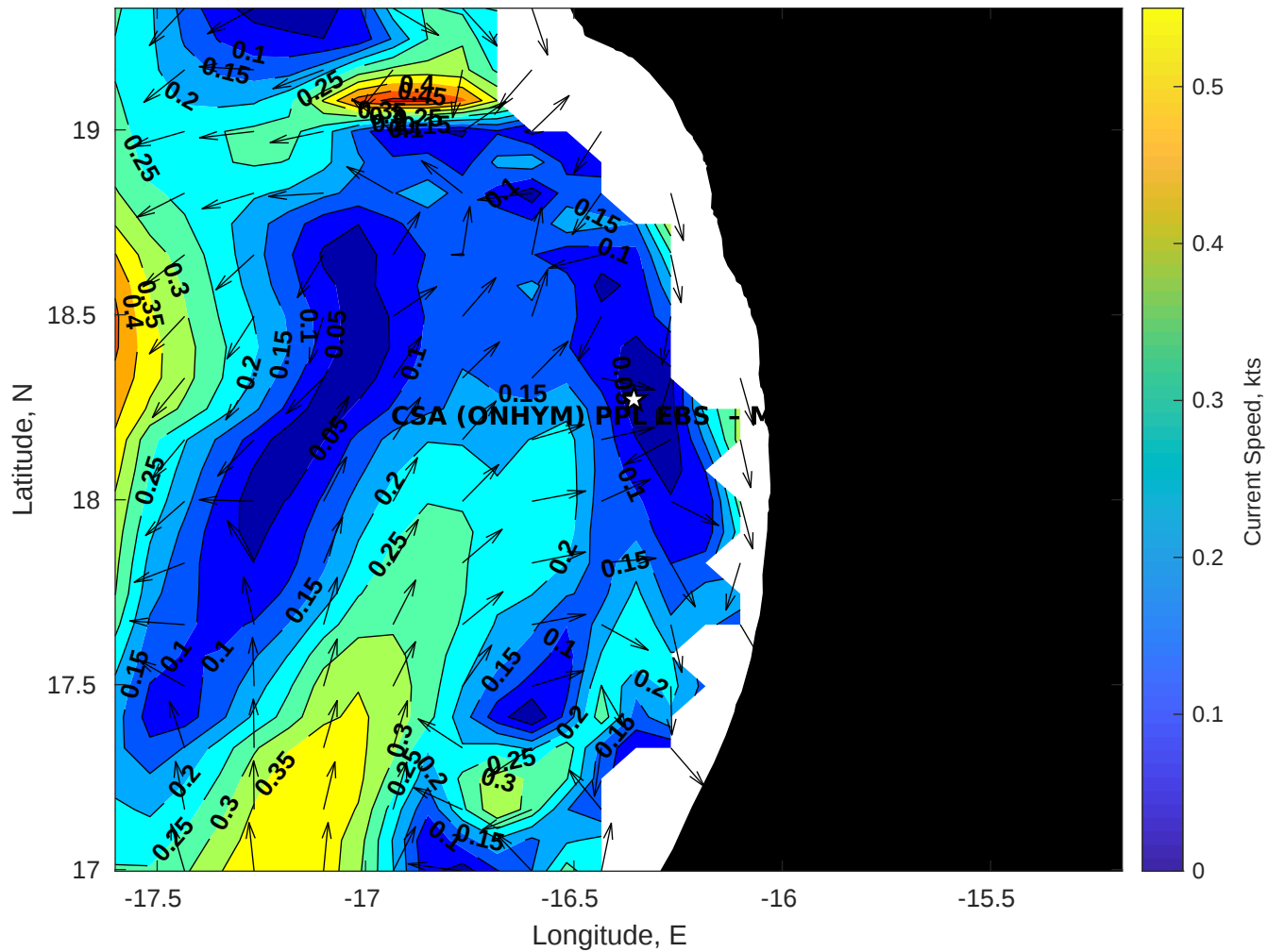
Surface Currents for CSA (ONHYM) PPL EBS - Mauritania at 21-Oct-2025 00:00:00
