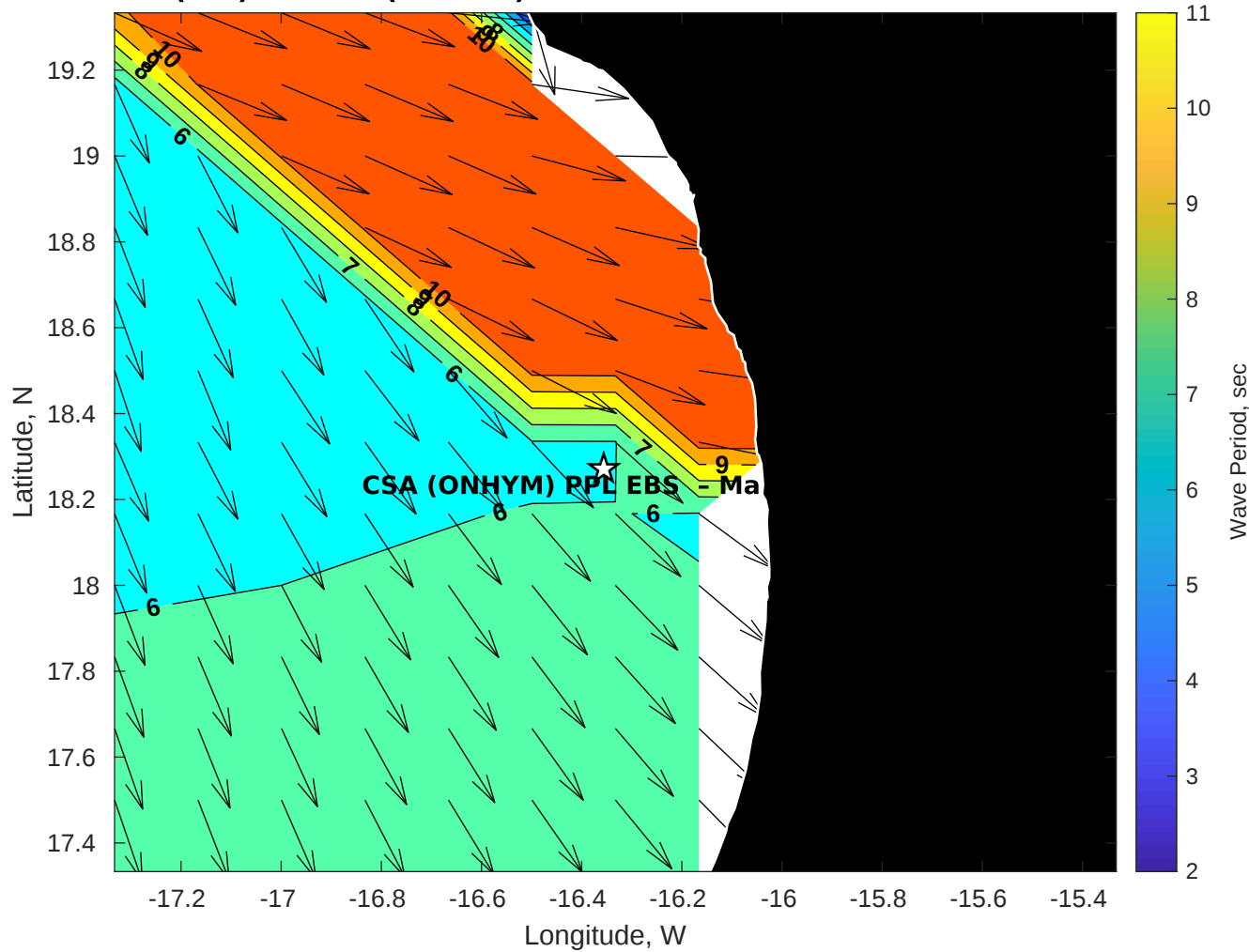
Wave Period (sec) for CSA (ONHYM) PPL EBS - Mauritania at 22-Oct-2025 09:00:00
