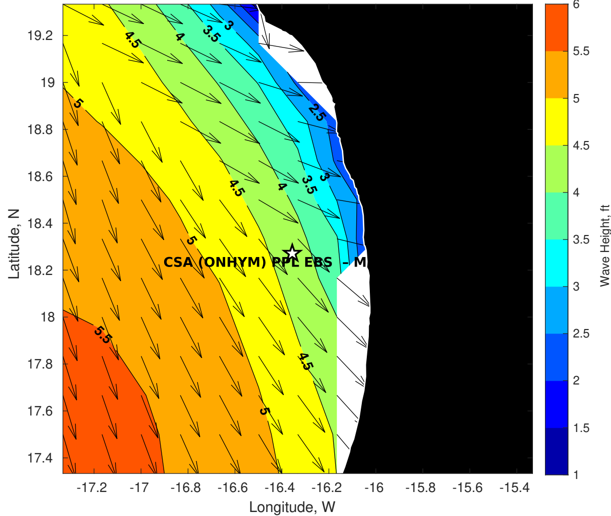
Wave Height (ft) for CSA (ONHYM) PPL EBS - Mauritania at 22-Oct-2025 09:00:00
