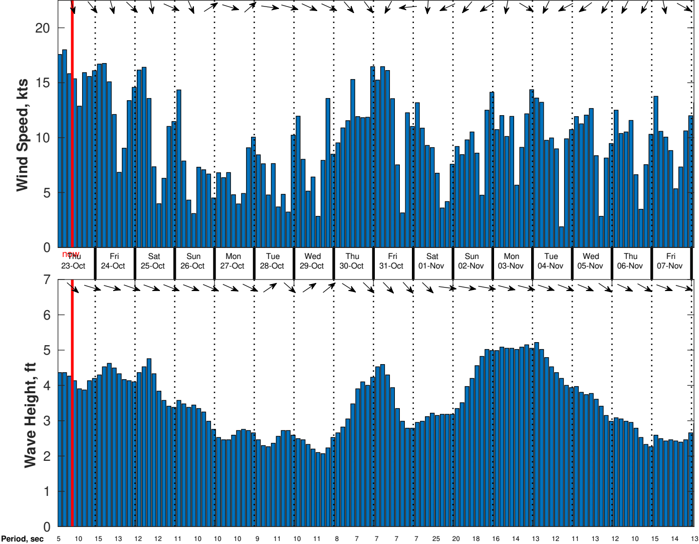
Wind & Wave Forecast for CSA (ONHYM) PPL EBS - Mauritania from 22-Oct-2025 01:00:00 to 07-Nov-2025 01:00:00
