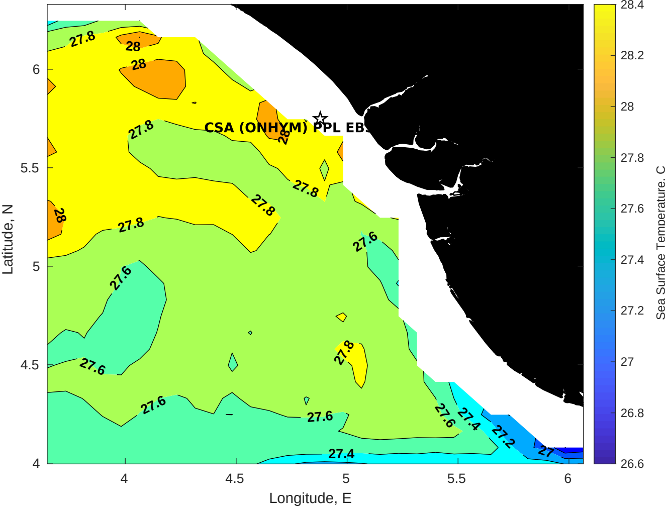
SST for CSA (ONHYM) PPL EBS - Nigeria at 21-Oct-2025 00:00:00
