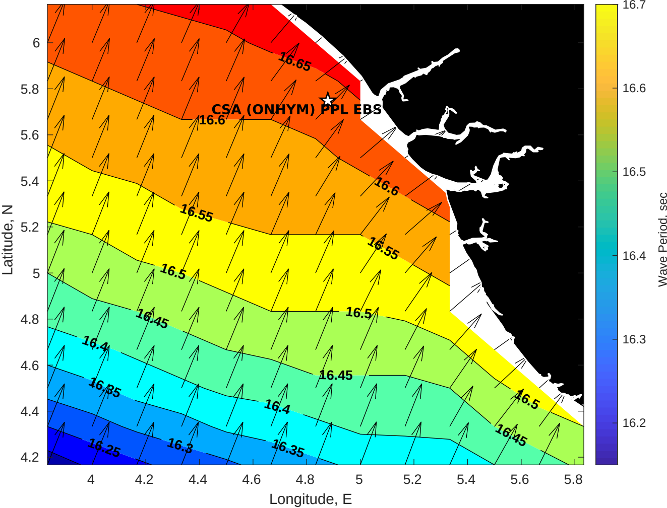
Wave Period (sec) for CSA (ONHYM) PPL EBS - Nigeria at 22-Oct-2025 09:00:00
