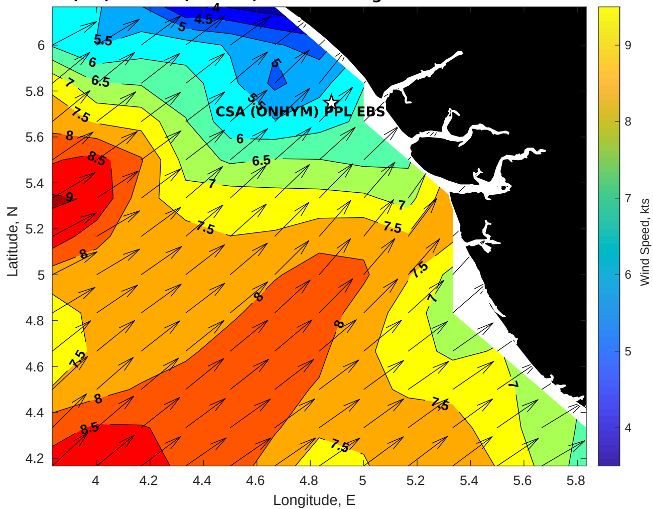
Winds (kts) for CSA (ONHYM) PPL EBS - Nigeria at 22-Oct-2025 09:00:00
