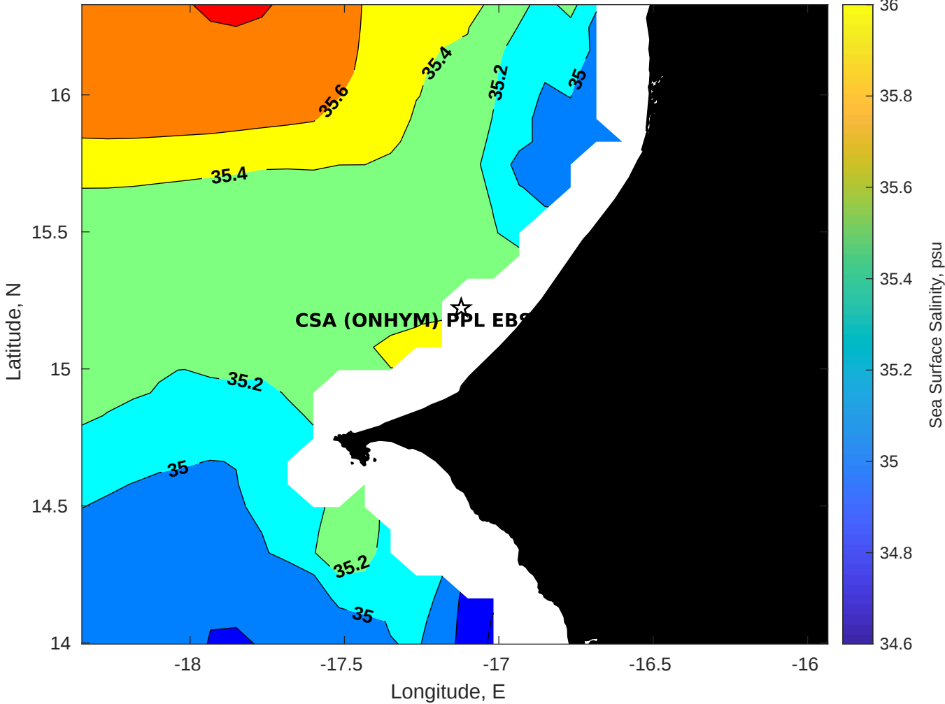
Surface Salinity for CSA (ONHYM) PPL EBS - Senegal at 21-Oct-2025 00:00:00
