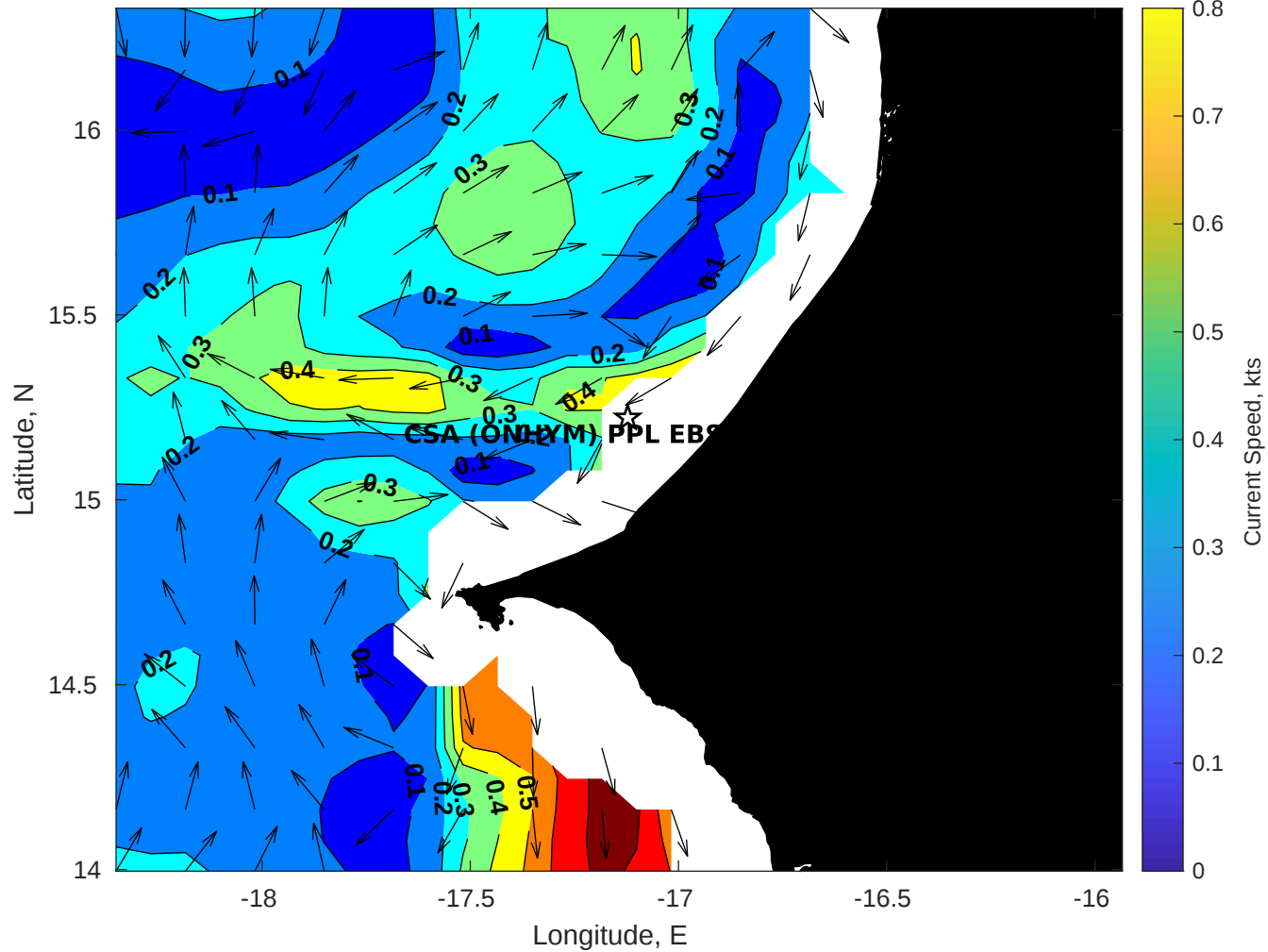
Surface Currents for CSA (ONHYM) PPL EBS - Senegal at 21-Oct-2025 00:00:00
