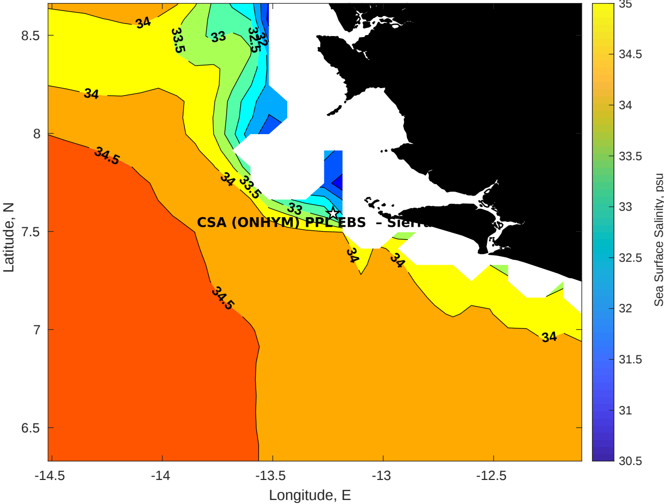
Surface Salinity for CSA (ONHYM) PPL EBS - Sierra Leone at 21-Oct-2025 00:00:00
