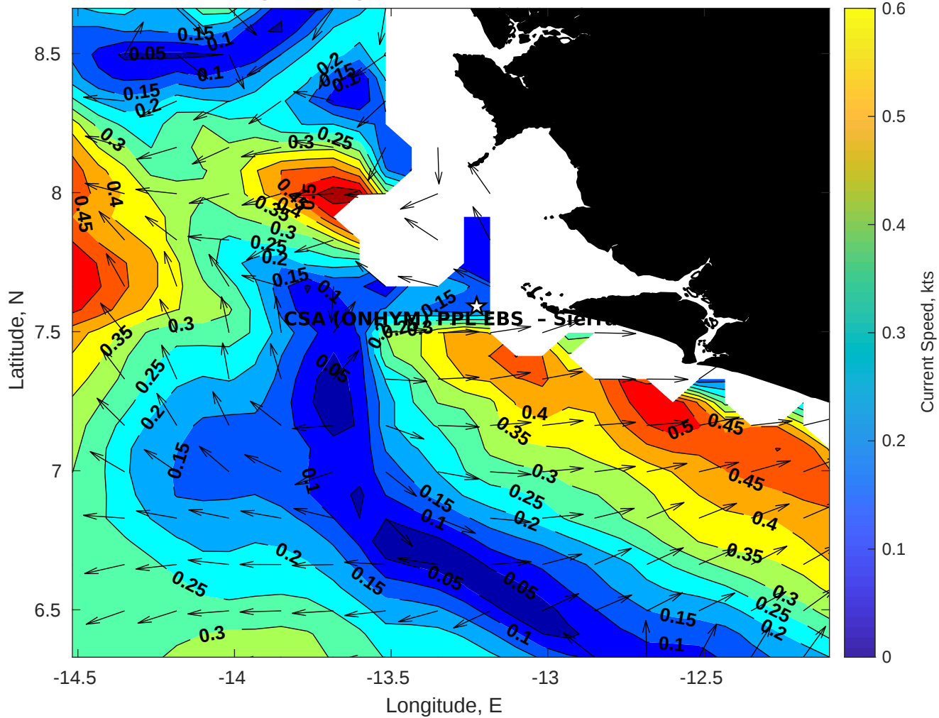
Surface Currents for CSA (ONHYM) PPL EBS - Sierra Leone at 21-Oct-2025 00:00:00
