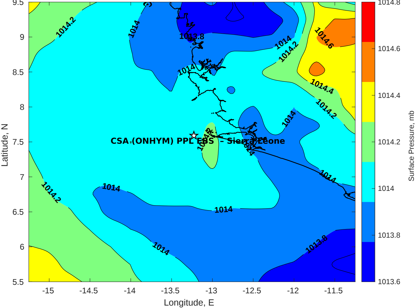
Surface Pressure (mb) for CSA (ONHYM) PPL EBS - Sierra Leone at 23-Oct-2025 00:00:00
