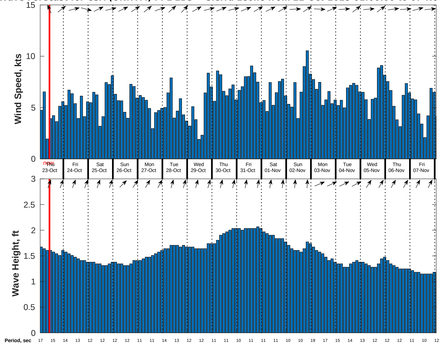
Wind & Wave Forecast for CSA (ONHYM) PPL EBS - Sierra Leone from 22-Oct-2025 01:00:00 to 07-Nov-2025 01:00:00
