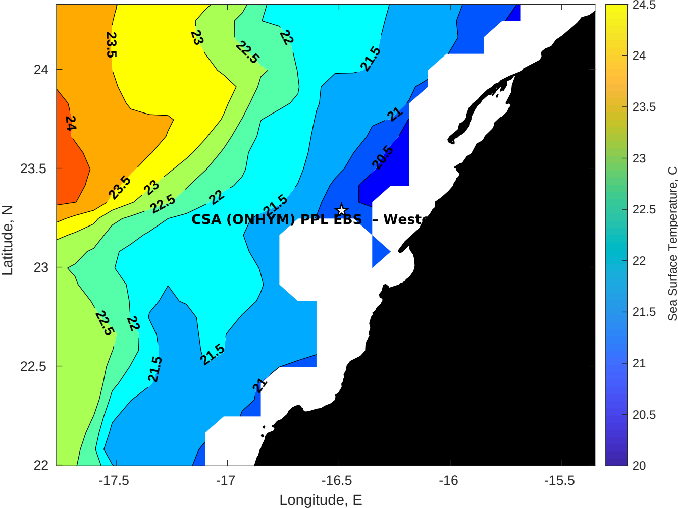
SST for CSA (ONHYM) PPL EBS - Western Sahara at 21-Oct-2025 00:00:00
