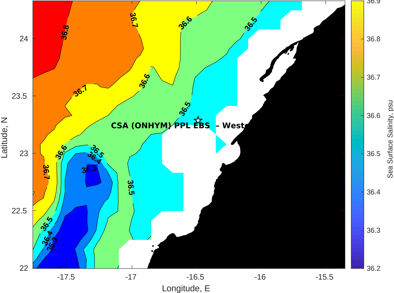
Surface Salinity for CSA (ONHYM) PPL EBS - Western Sahara at 21-Oct-2025 00:00:00
