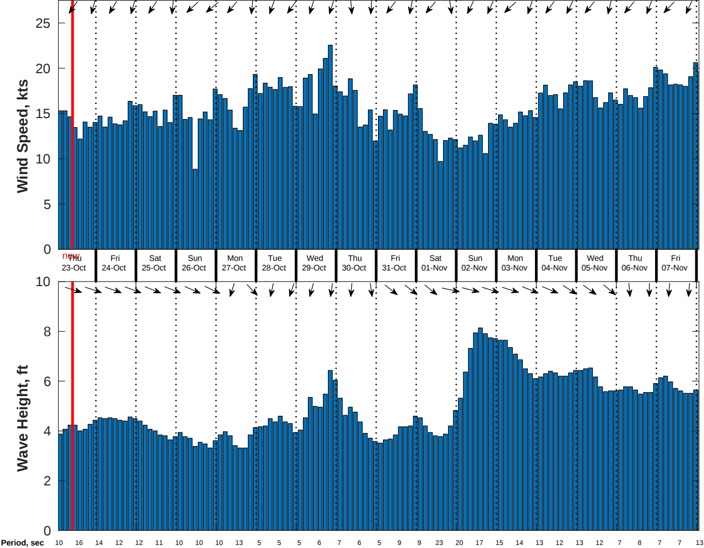
Wind & Wave Forecast for CSA (ONHYM) PPL EBS - Western Sahara from 22-Oct-2025 01:00:00 to 07-Nov-2025 01:00:00
