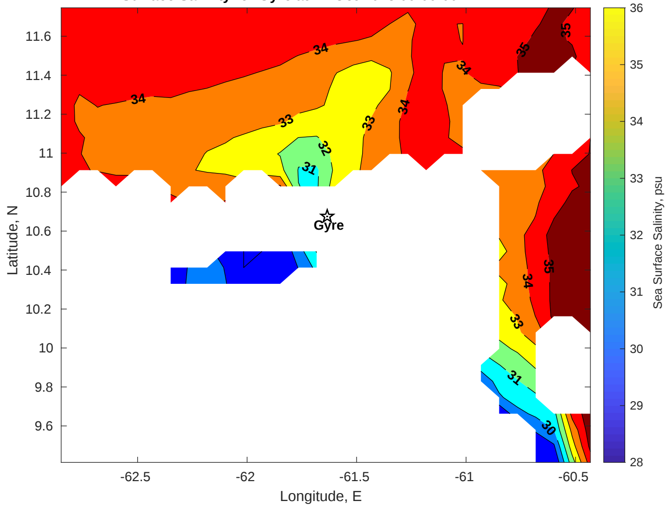
Surface Salinity for Gyre at 21-Oct-2025 00:00:00
