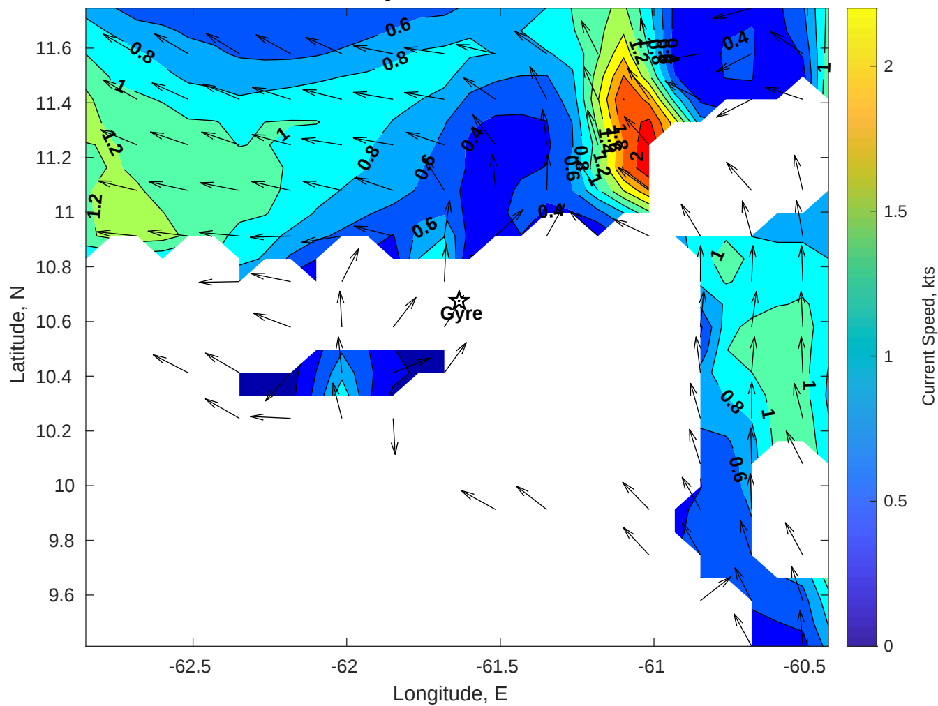
Surface Currents for Gyre at 21-Oct-2025 00:00:00
