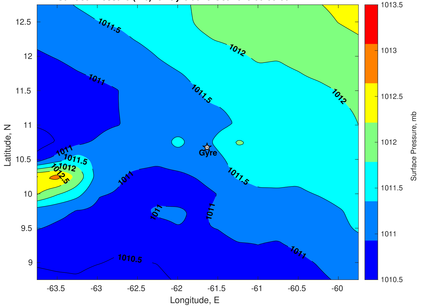
Surface Pressure (mb) for Gyre at 23-Oct-2025 00:00:00
