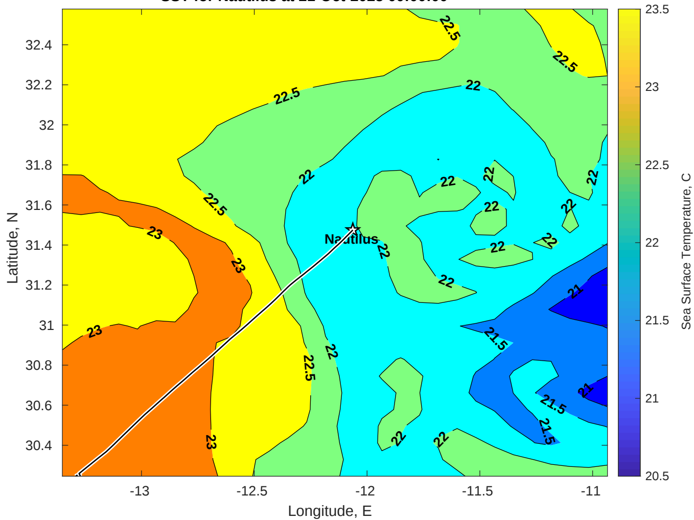
SST for Nautilus at 21-Oct-2025 00:00:00
