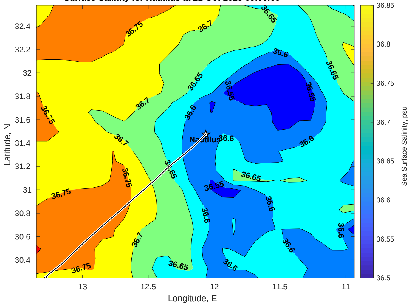
Surface Salinity for Nautilus at 21-Oct-2025 00:00:00
