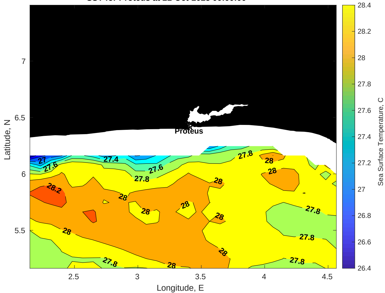
SST for Proteus at 21-Oct-2025 00:00:00
