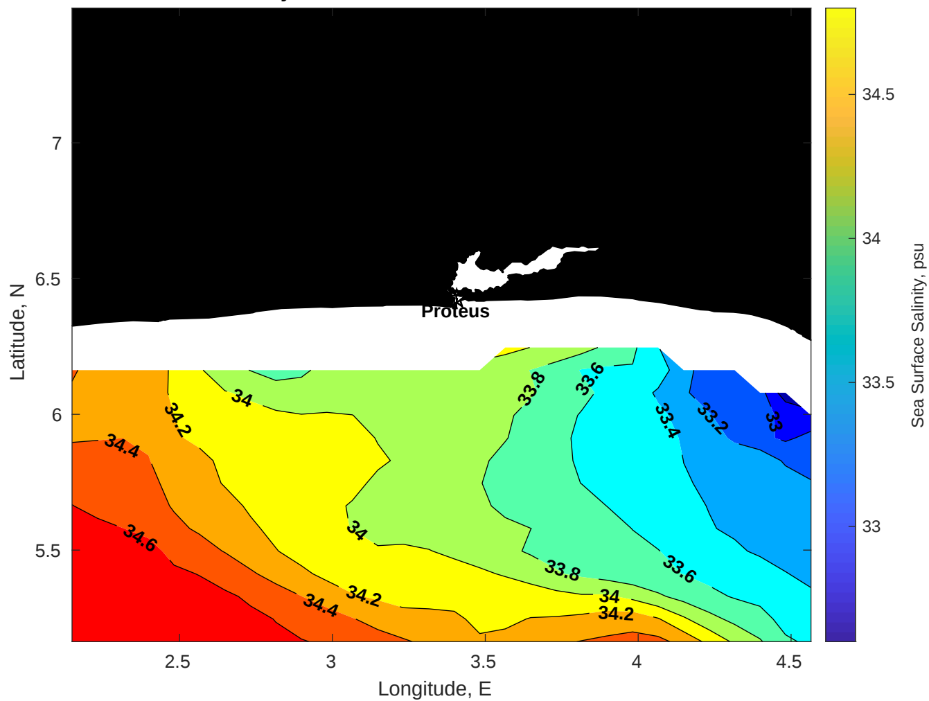
Surface Salinity for Proteus at 21-Oct-2025 00:00:00
