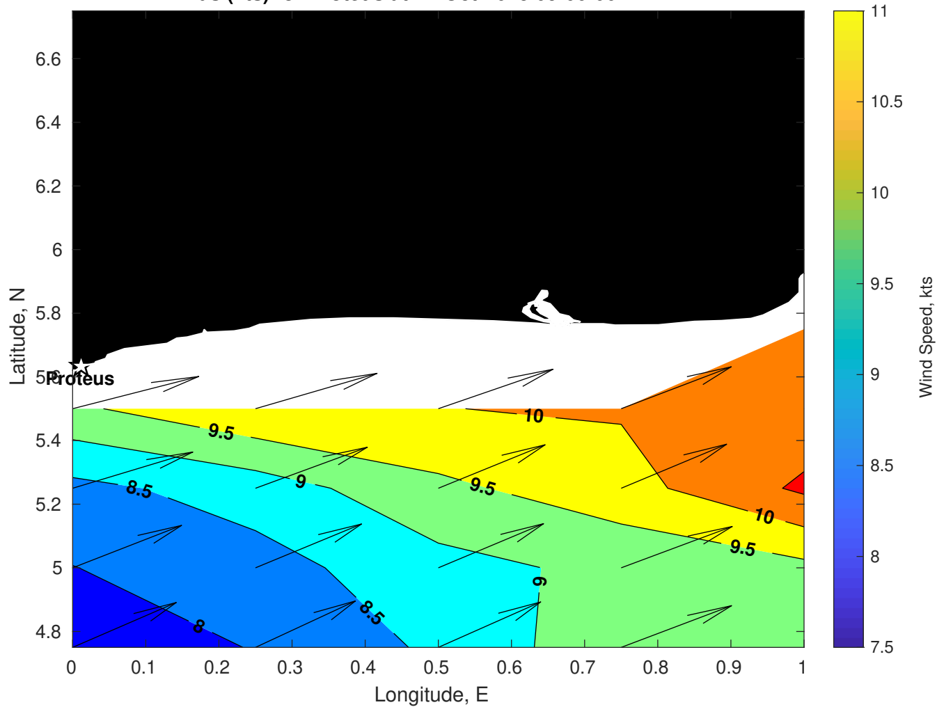
Winds (kts) for Proteus at 22-Oct-2025 09:00:00
