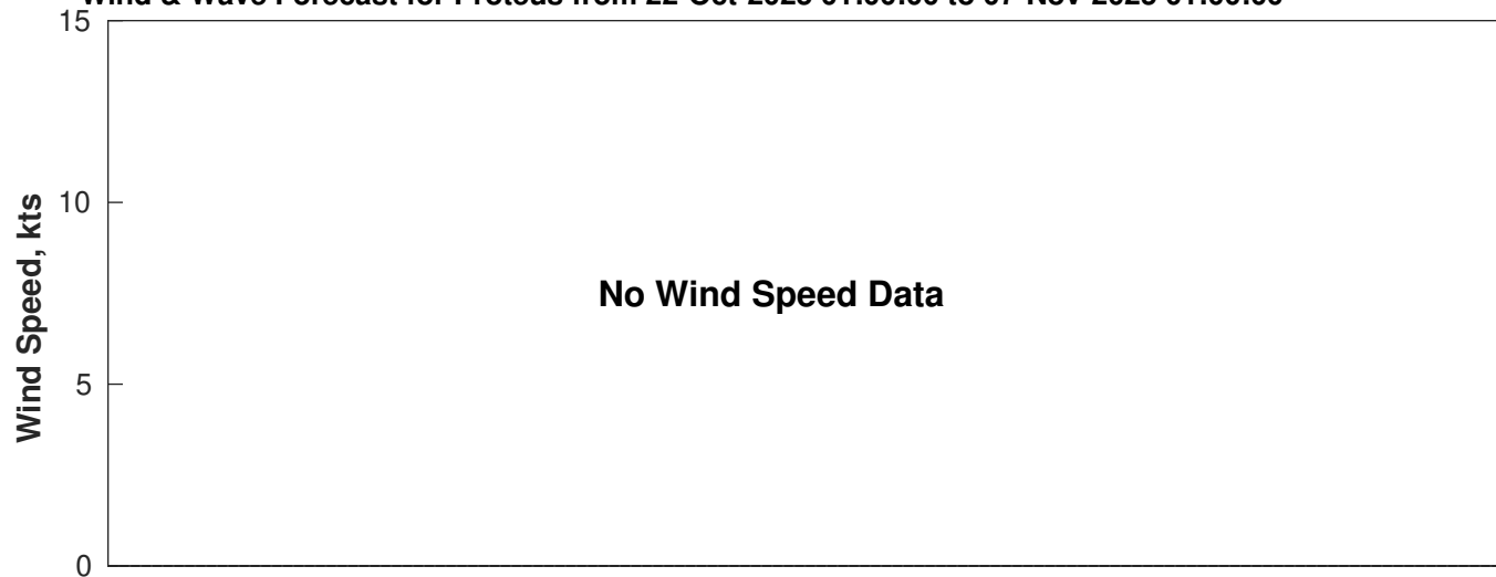
Wind & Wave Forecast for Proteus from 22-Oct-2025 01:00:00 to 07-Nov-2025 01:00:00
