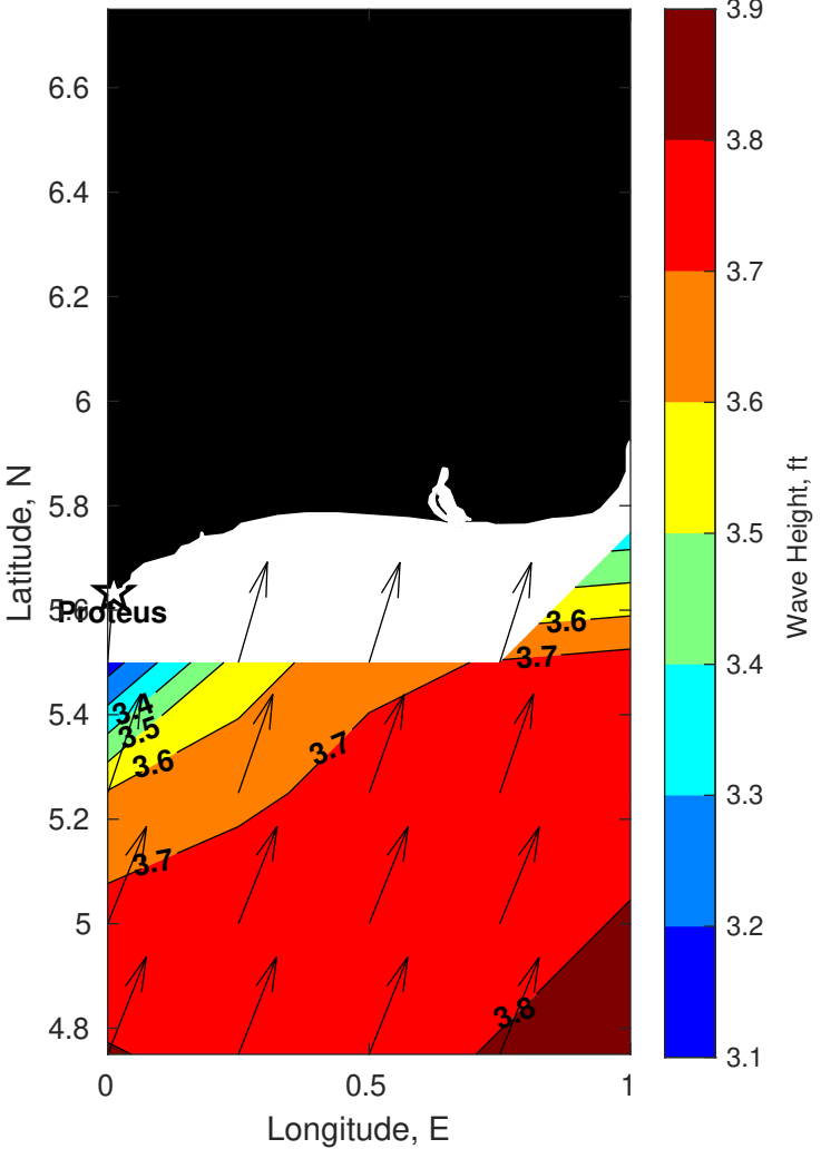
Wave Height (ft) for Proteus at 22-Oct-2025 09:00:00
