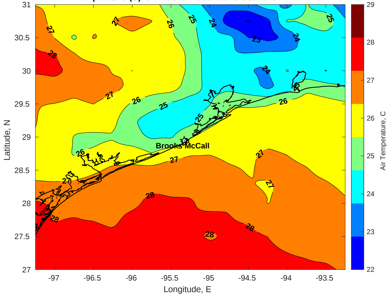
Air Temperature (C) for Brooks McCall at 23-Oct-2025
