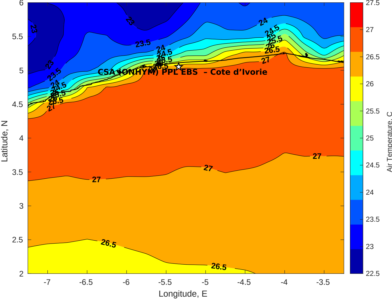
Air Temperature (C) for CSA (ONHYM) PPL EBS - Cote d'Ivoire at 23-Oct-2025
