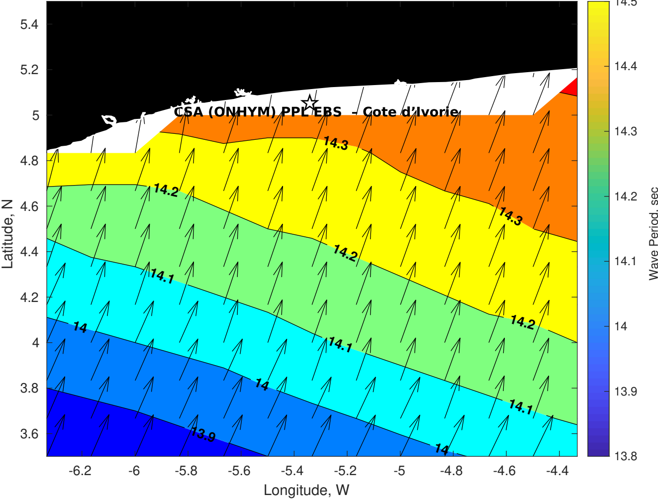
Wave Period (sec) for CSA (ONHYM) PPL EBS - Cote d'Ivoire at 22-Oct-2025 21:00:00
