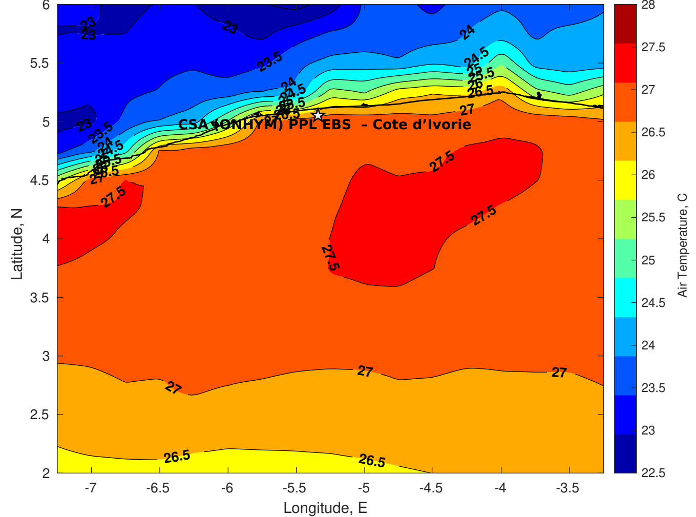
Air Temperature (C) for CSA (ONHYM) PPL EBS - Cote d'Ivoire at 23-Oct-2025
