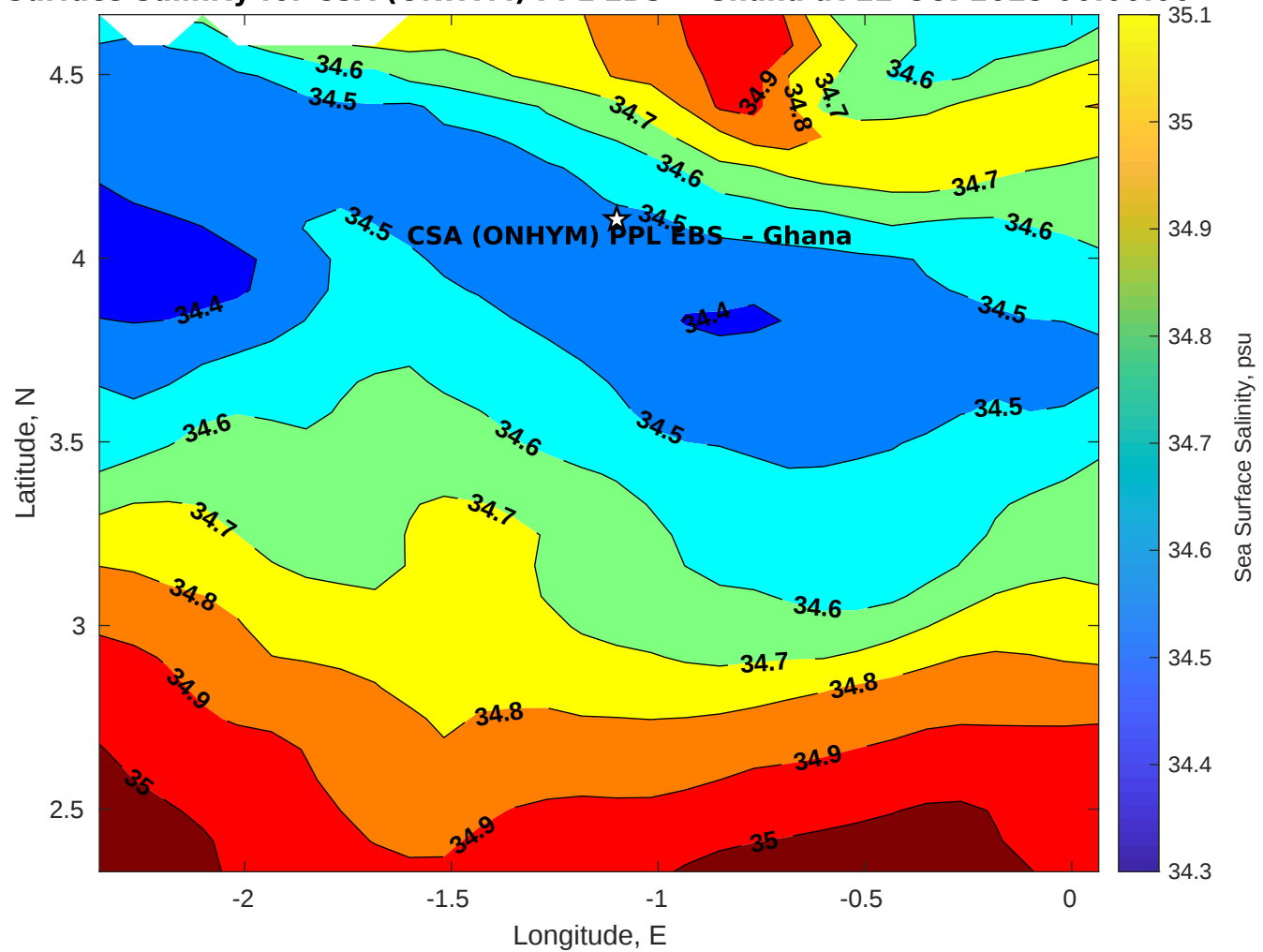
Surface Salinity for CSA (ONHYM) PPL EBS - Ghana at 22-Oct-2025 00:00:00
