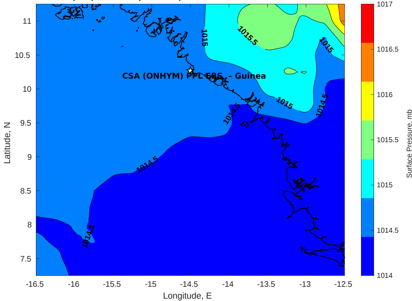
Surface Pressure (mb) for CSA (ONHYM) PPL EBS - Guinea at 23-Oct-2025 00:00:00
