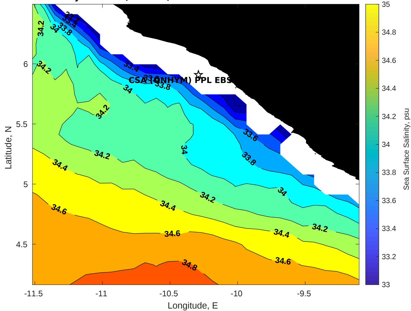
Surface Salinity for CSA (ONHYM) PPL EBS - Liberia at 22-Oct-2025 00:00:00
