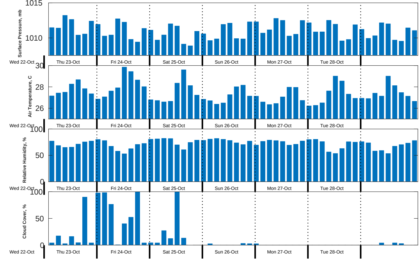
Met Forecast for CSA (ONHYM) PPL EBS - Mauritania from 23-Oct-2025 00:00:00 to 30-Oct-2025 00:00:00
