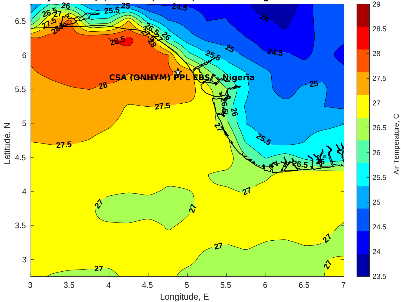
Air Temperature (C) for CSA (ONHYM) PPL EBS - Nigeria at 23-Oct-2025
