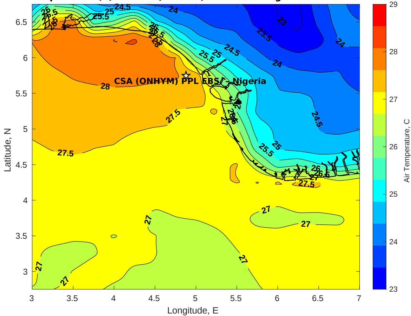
Air Temperature (C) for CSA (ONHYM) PPL EBS - Nigeria at 23-Oct-2025
