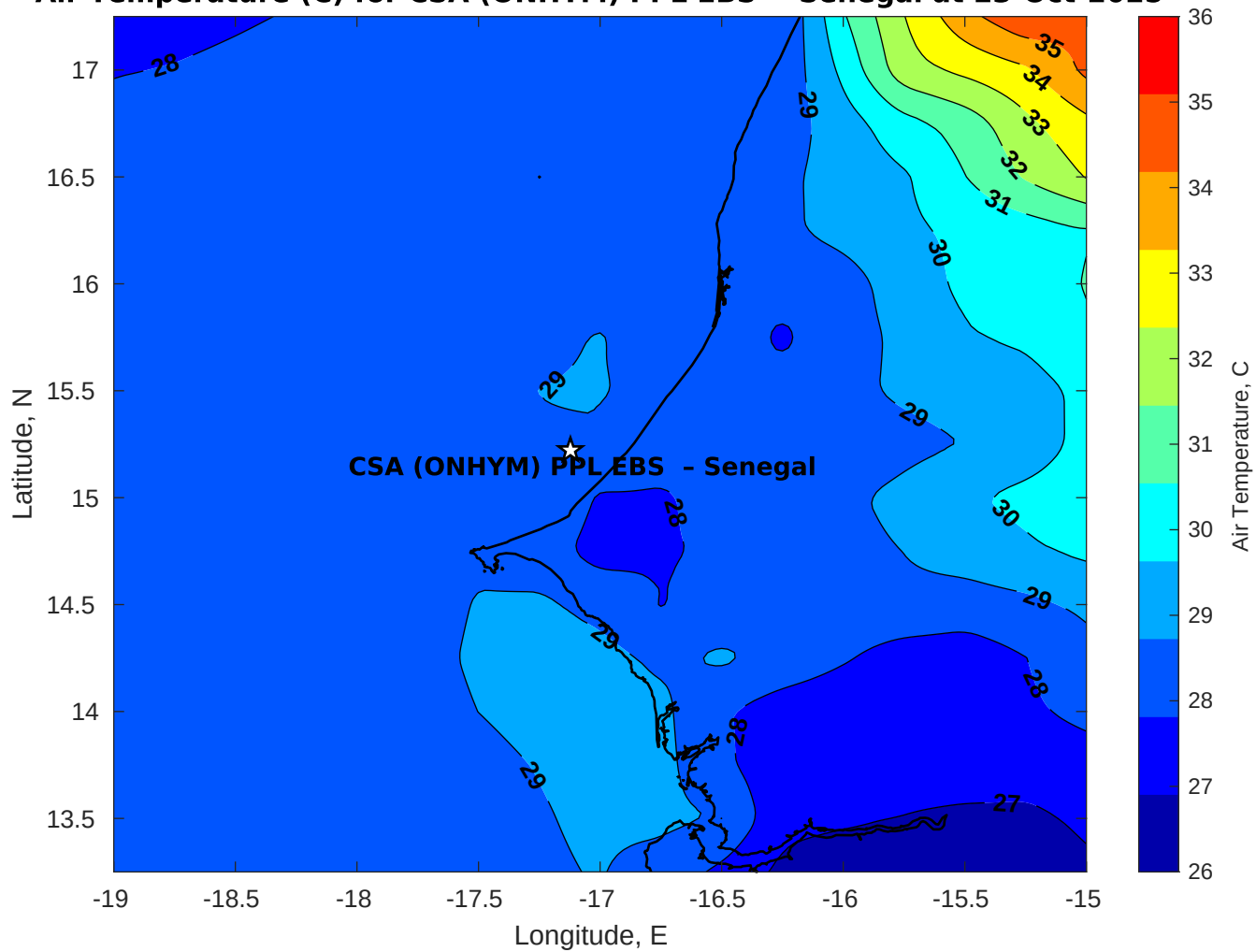
Air Temperature (C) for CSA (ONHYM) PPL EBS - Senegal at 23-Oct-2025
