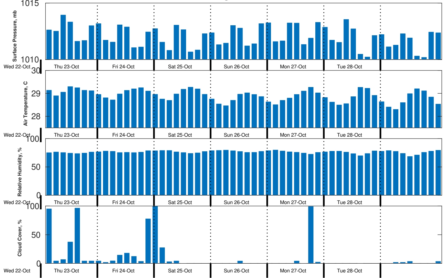
Met Forecast for CSA (ONHYM) PPL EBS - Senegal from 23-Oct-2025 00:00:00 to 30-Oct-2025 00:00:00
