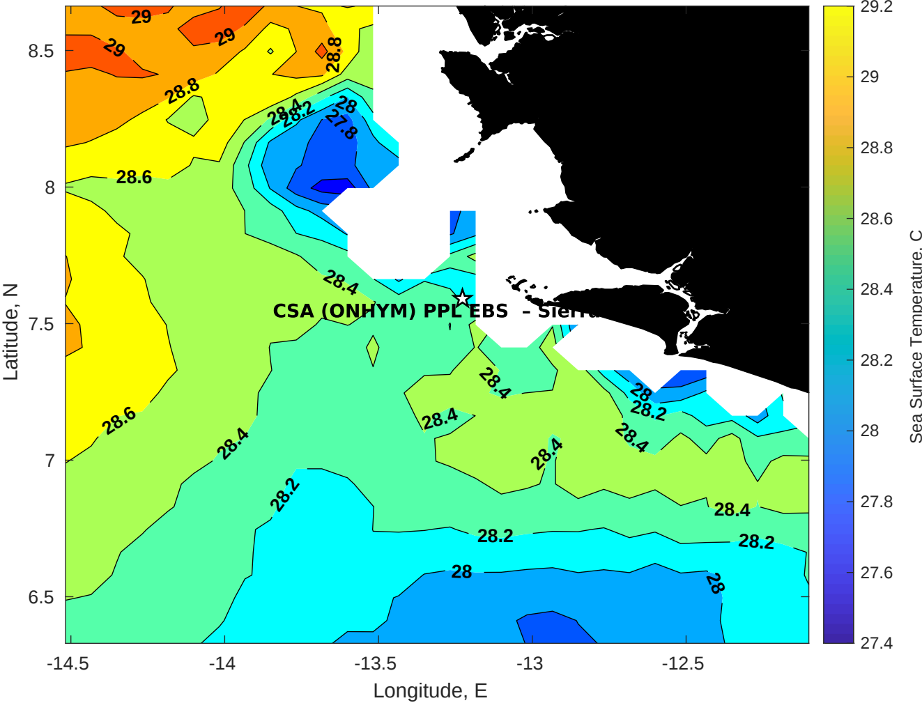
SST for CSA (ONHYM) PPL EBS - Sierra Leone at 22-Oct-2025 00:00:00
