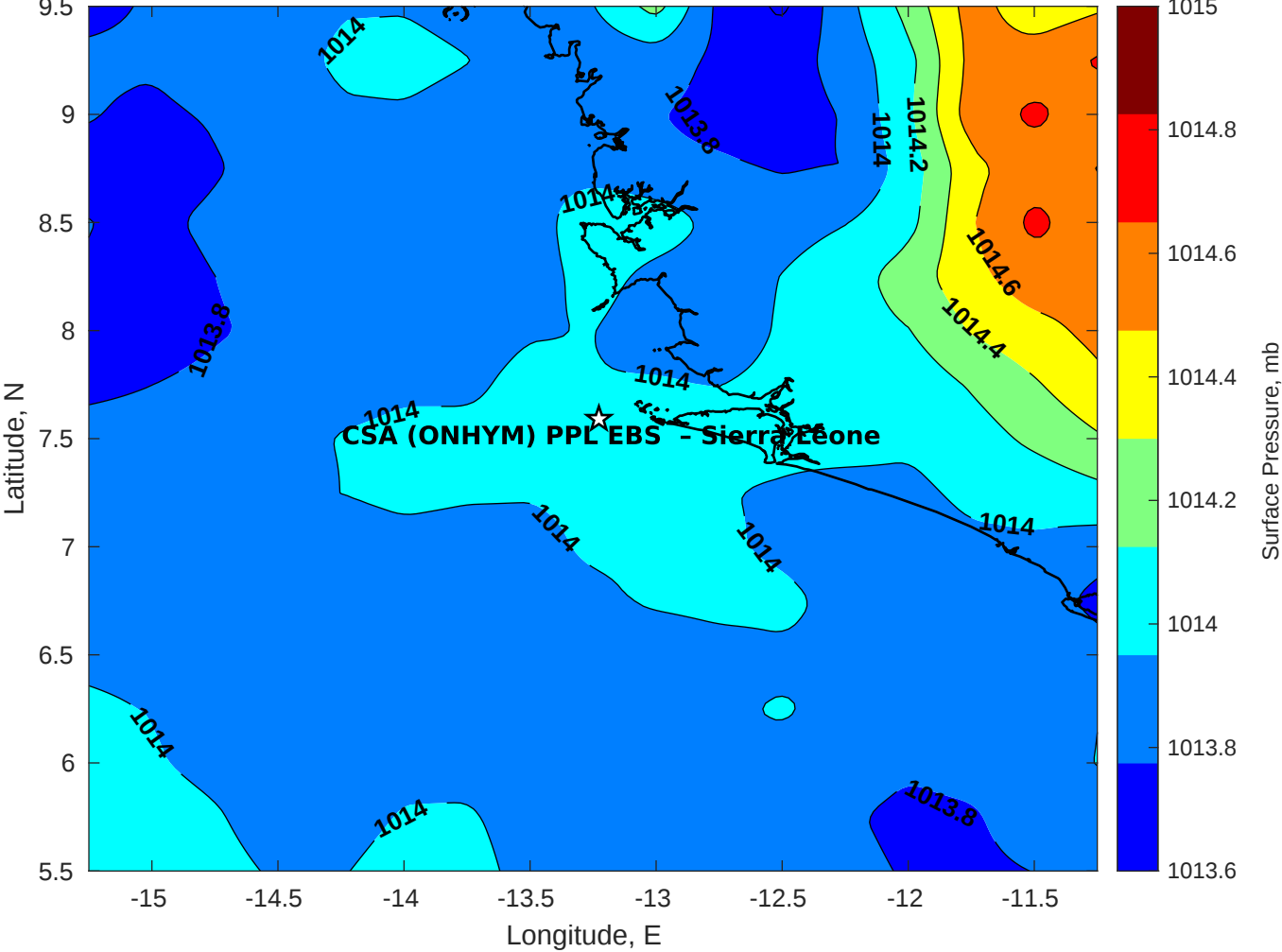
Surface Pressure (mb) for CSA (ONHYM) PPL EBS - Sierra Leone at 25-Oct-2025 00:00:00
