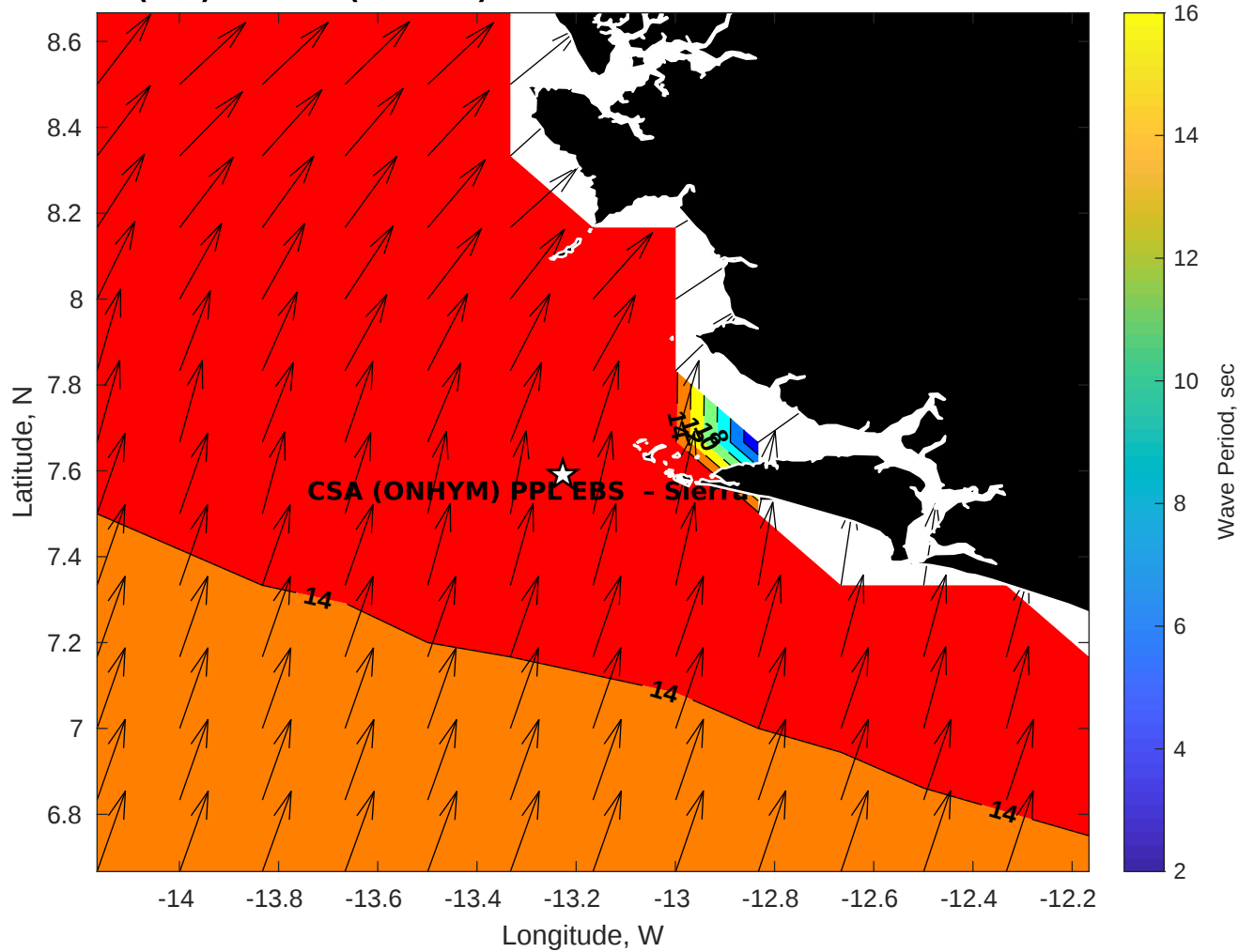
Wave Period (sec) for CSA (ONHYM) PPL EBS - Sierra Leone at 22-Oct-2025 21:00:00
