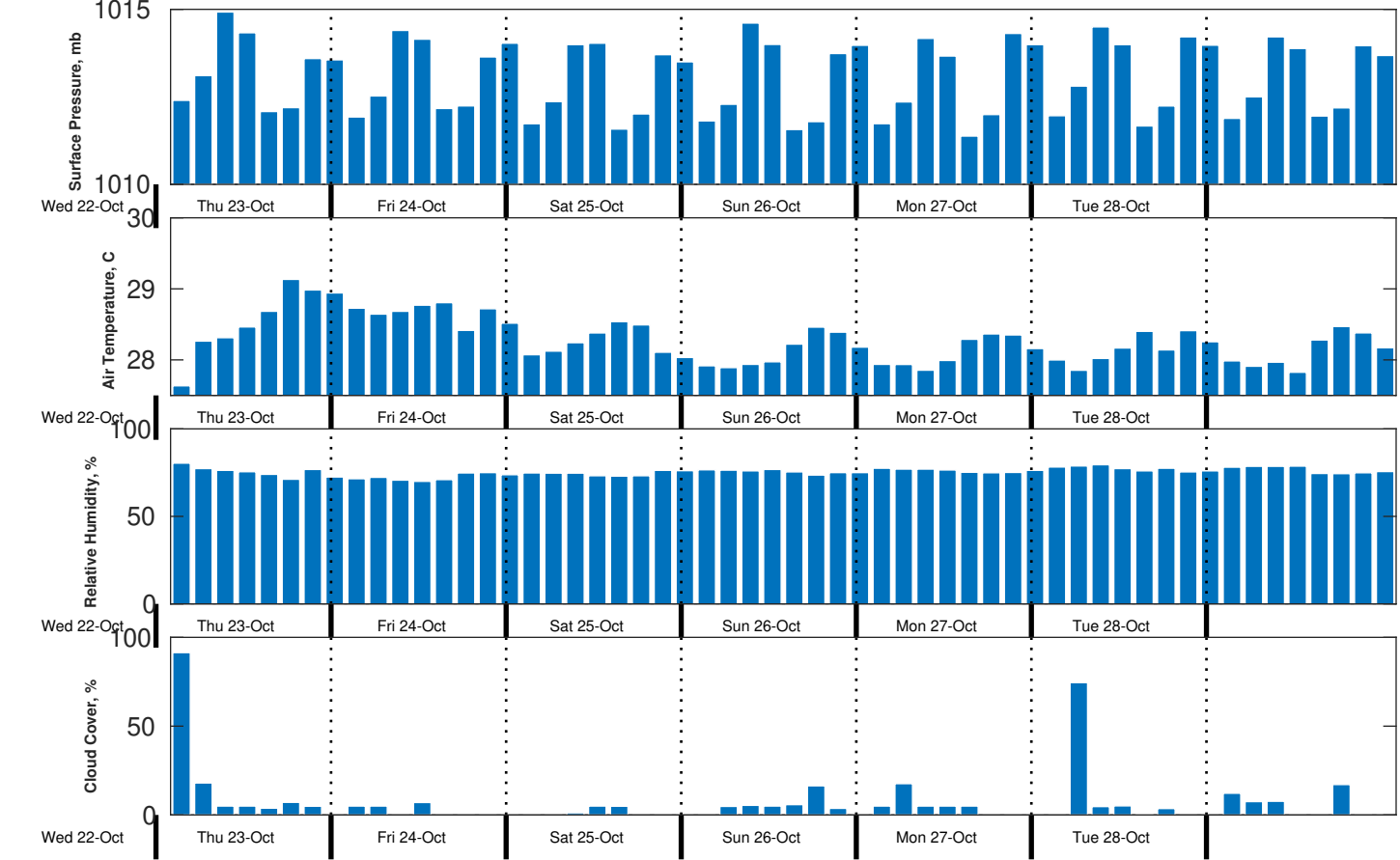
Met Forecast for CSA (ONHYM) PPL EBS - Sierra Leone from 23-Oct-2025 00:00:00 to 30-Oct-2025 00:00:00
