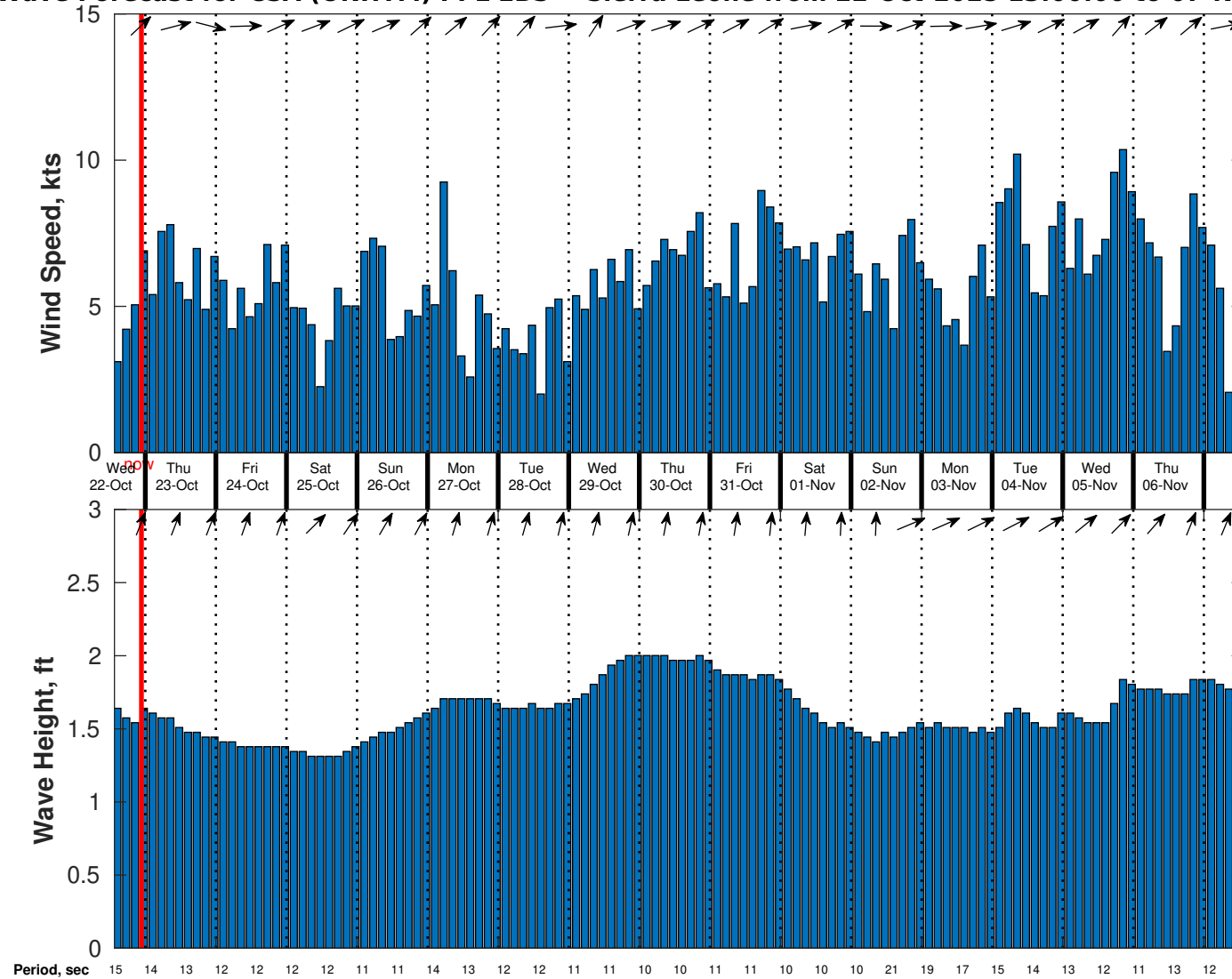
Wind & Wave Forecast for CSA (ONHYM) PPL EBS - Sierra Leone from 22-Oct-2025 13:00:00 to 07-Nov-2025 13:00:00
