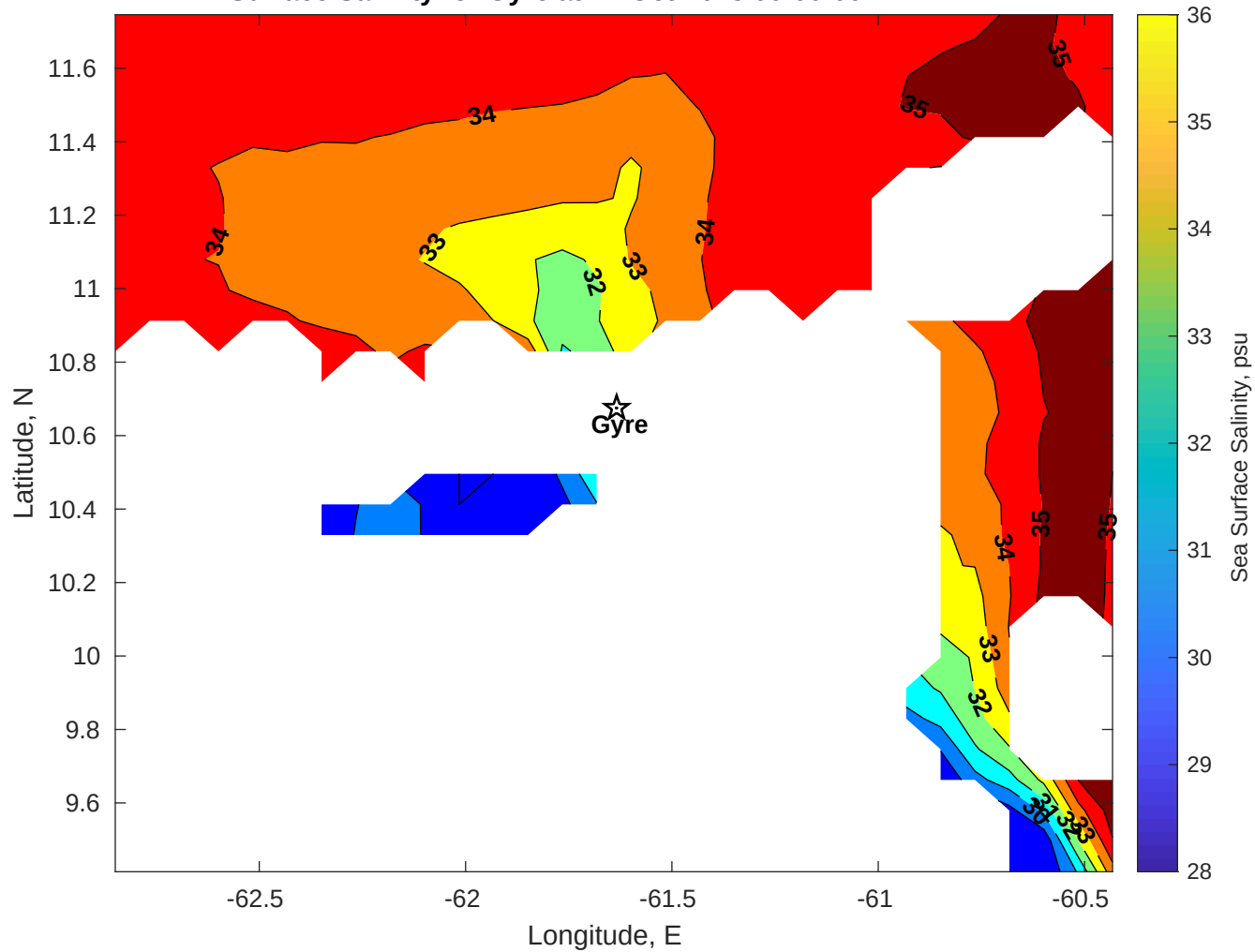
Surface Salinity for Gyre at 22-Oct-2025 00:00:00
