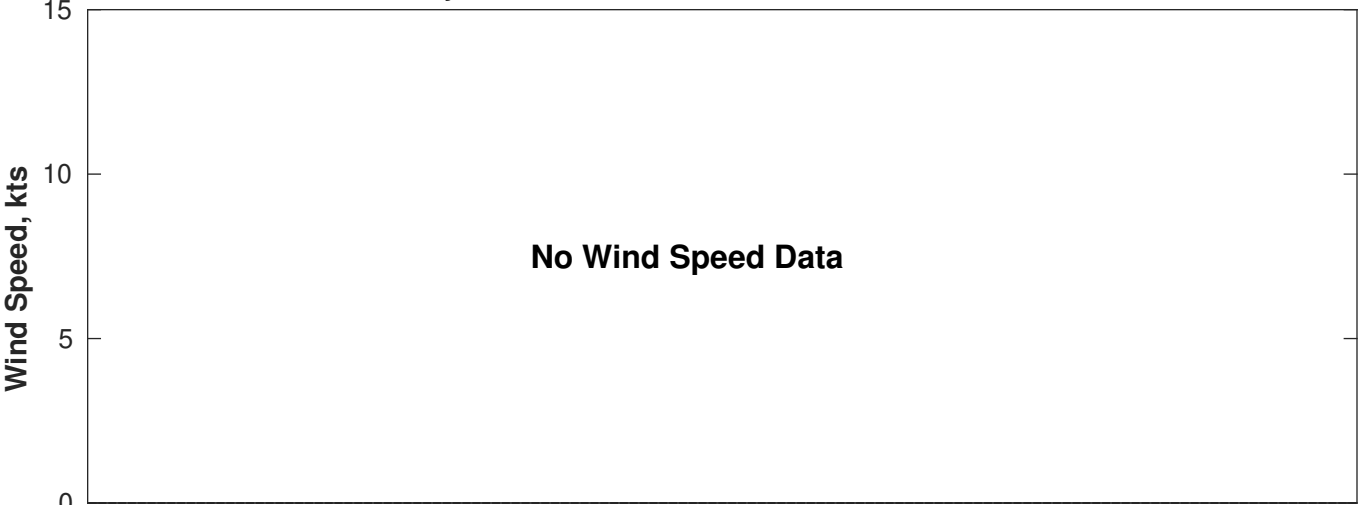
Wind & Wave Forecast for Gyre from 22-Oct-2025 20:00:00 to 07-Nov-2025 20:00:00
