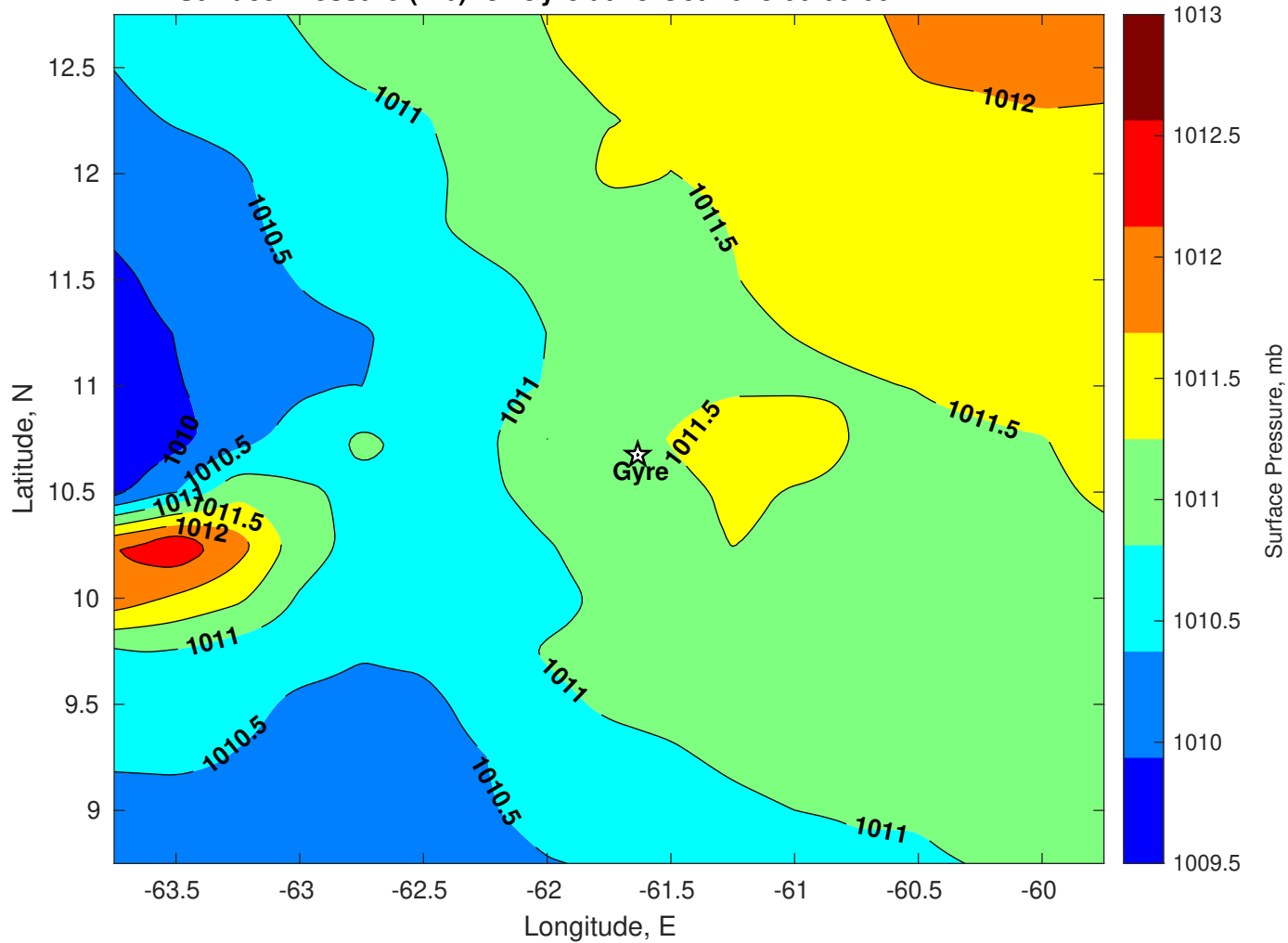
Surface Pressure (mb) for Gyre at 25-Oct-2025 00:00:00
