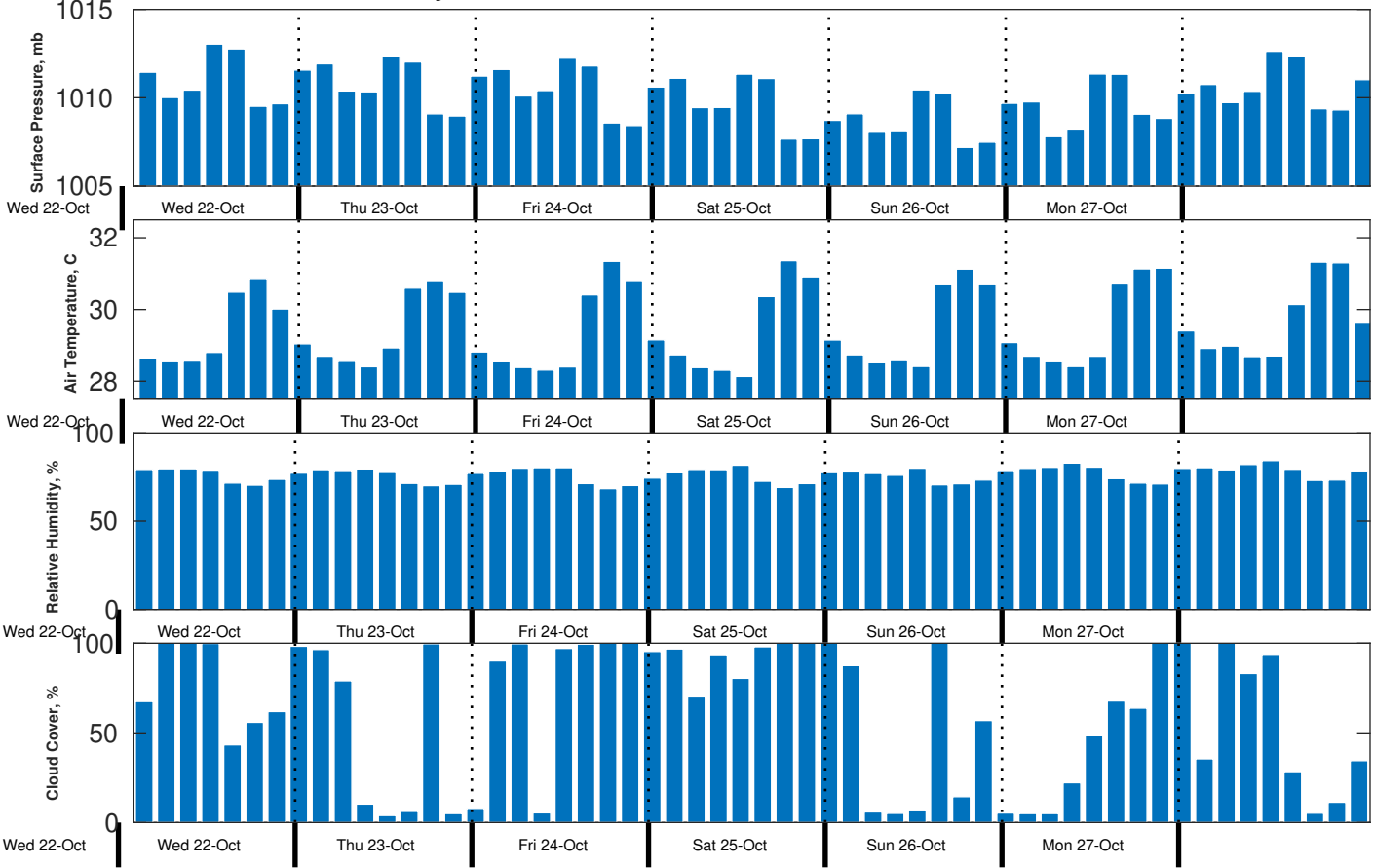
Met Forecast for Gyre from 22-Oct-2025 20:00:00 to 29-Oct-2025 20:00:00
