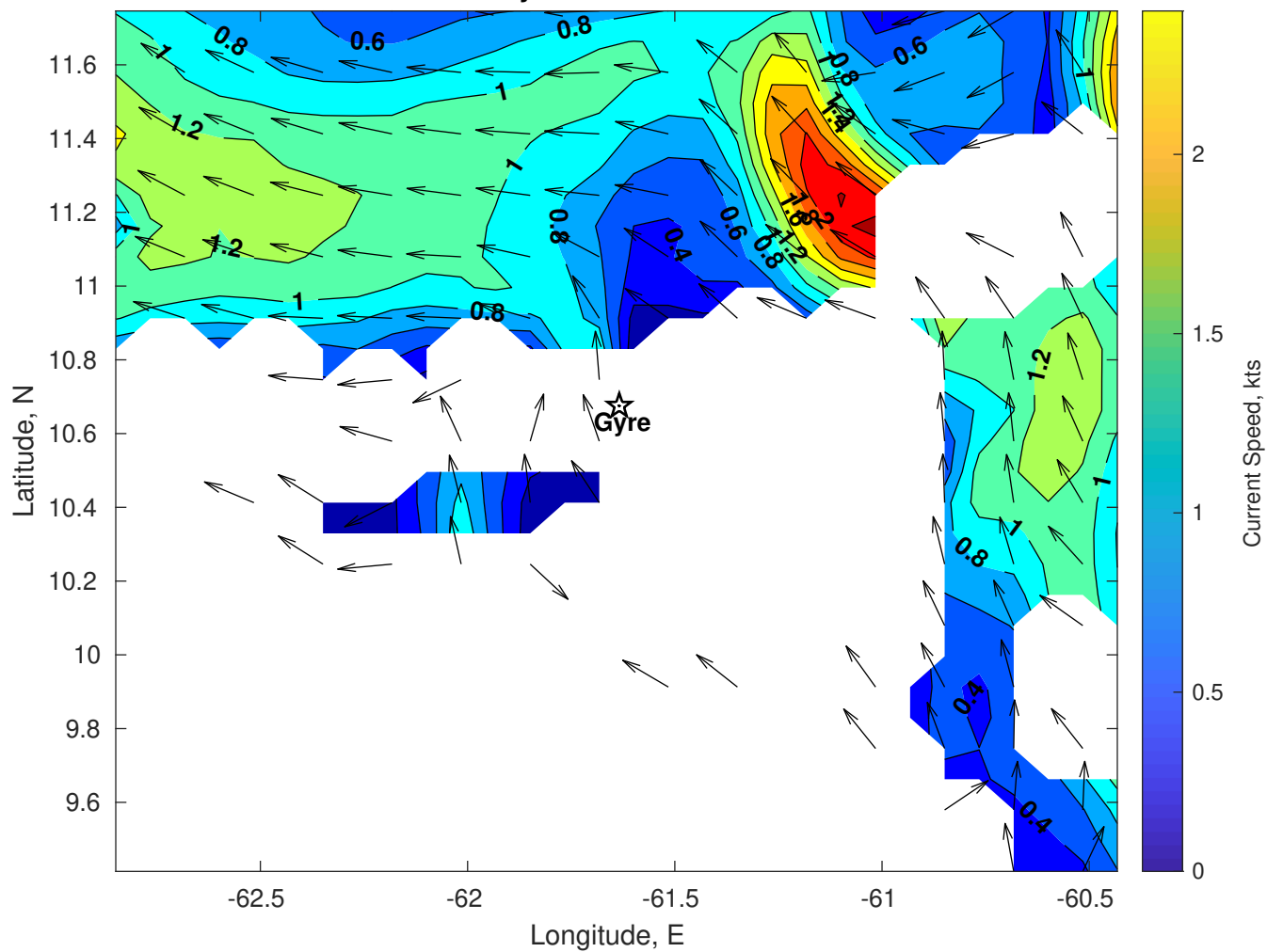
Surface Currents for Gyre at 22-Oct-2025 00:00:00
