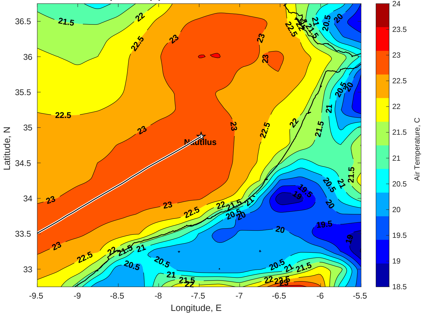
Air Temperature (C) for Nautilus at 23-Oct-2025
