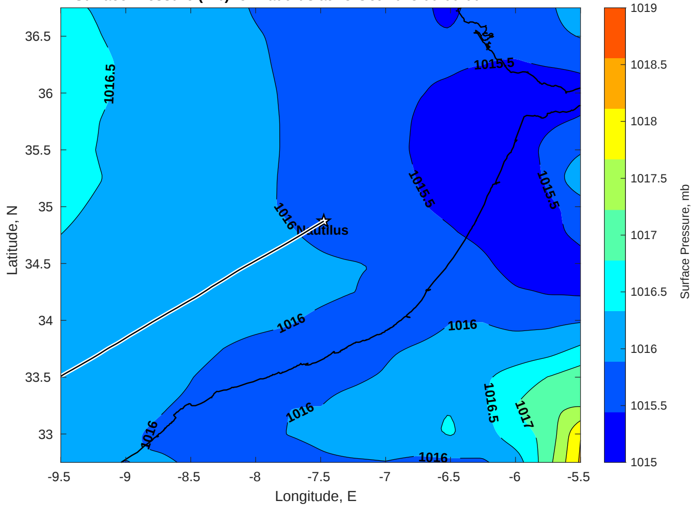
Surface Pressure (mb) for Nautilus at 25-Oct-2025 00:00:00
