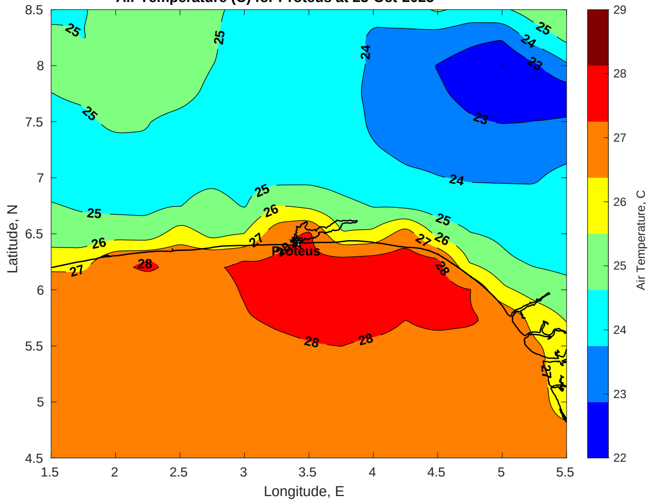
Air Temperature (C) for Proteus at 23-Oct-2025
