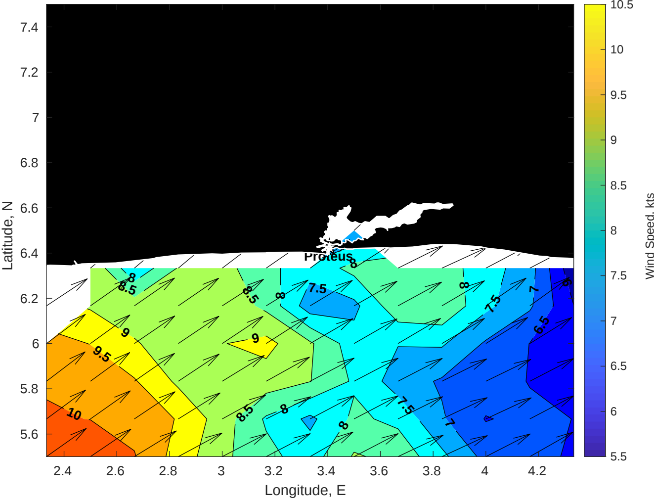
Winds (kts) for Proteus at 23-Oct-2025 09:00:00
