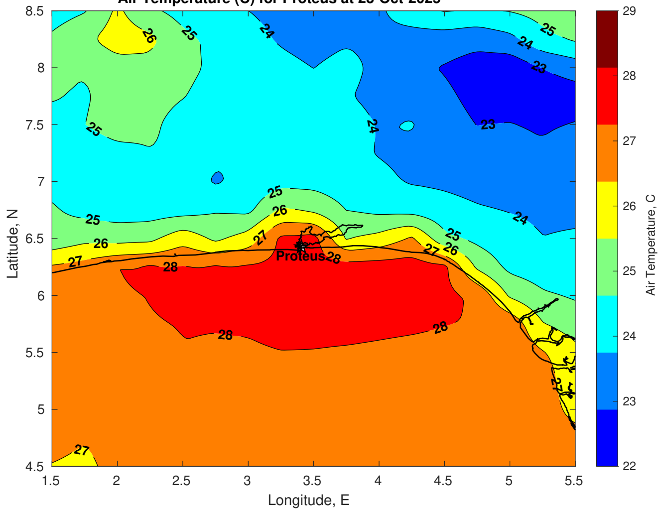
Air Temperature (C) for Proteus at 23-Oct-2025
