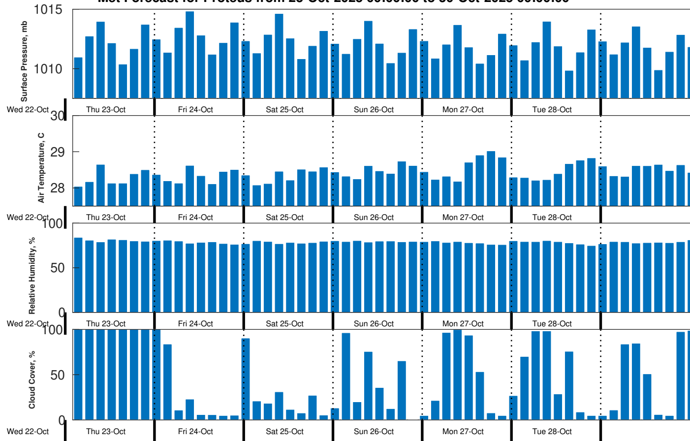
Met Forecast for Proteus from 23-Oct-2025 00:00:00 to 30-Oct-2025 00:00:00
