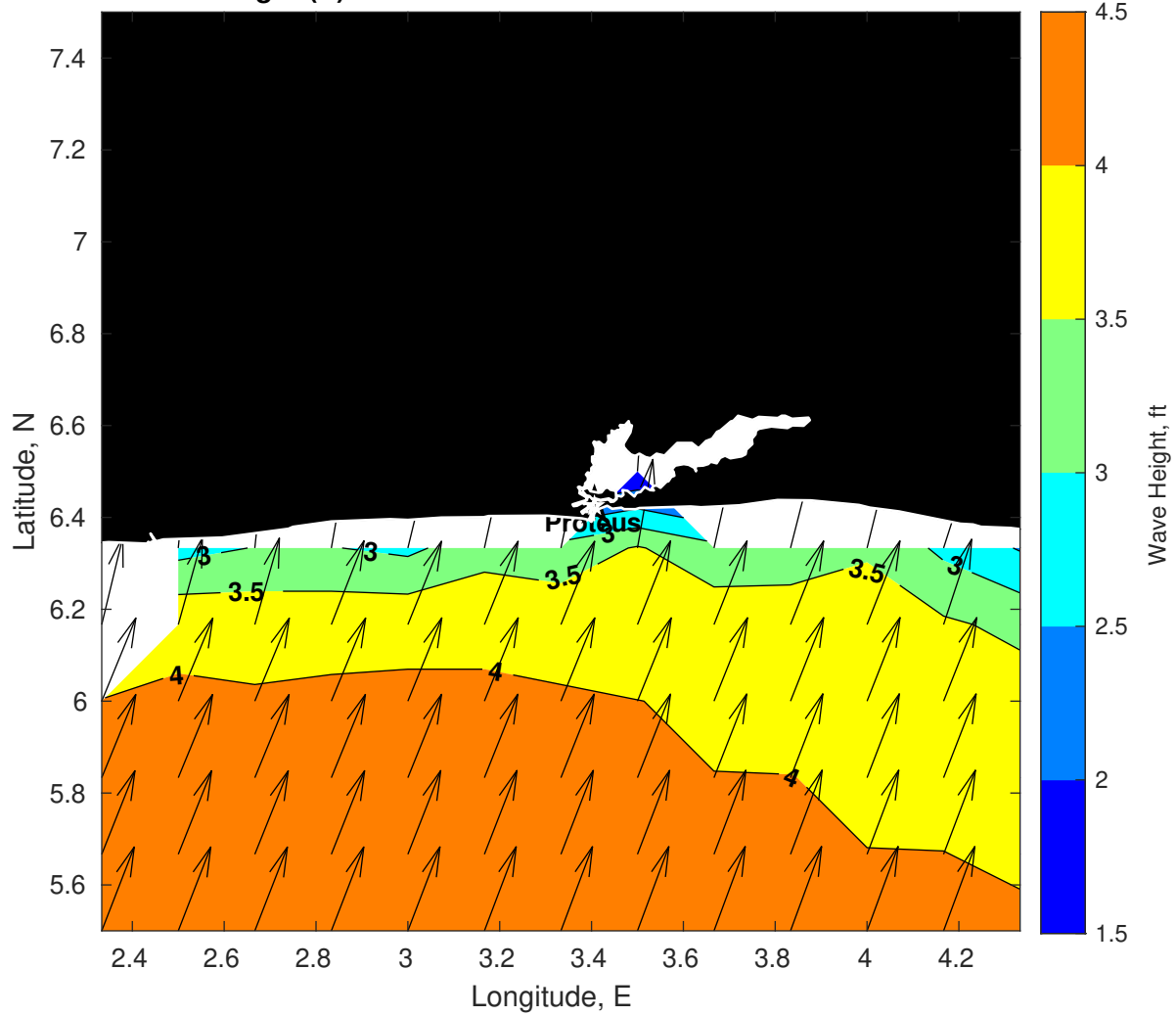
Wave Height (ft) for Proteus at 23-Oct-2025 09:00:00
