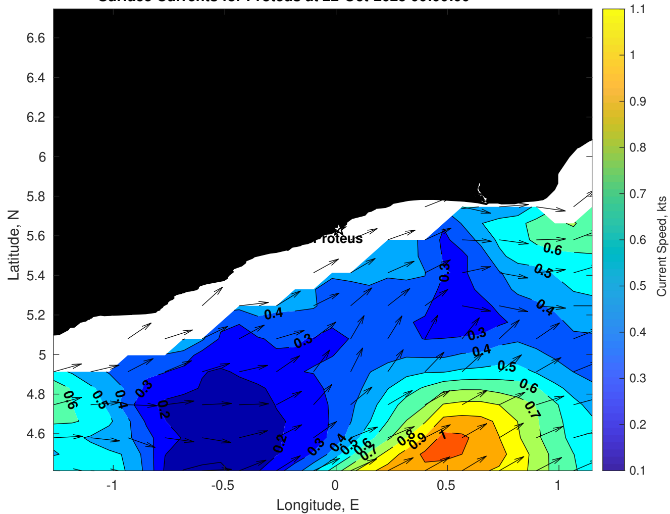
Surface Currents for Proteus at 22-Oct-2025 00:00:00
