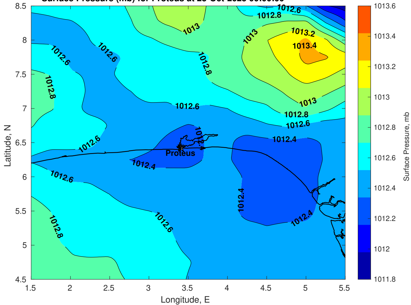
Surface Pressure (mb) for Proteus at 23-Oct-2025 00:00:00
