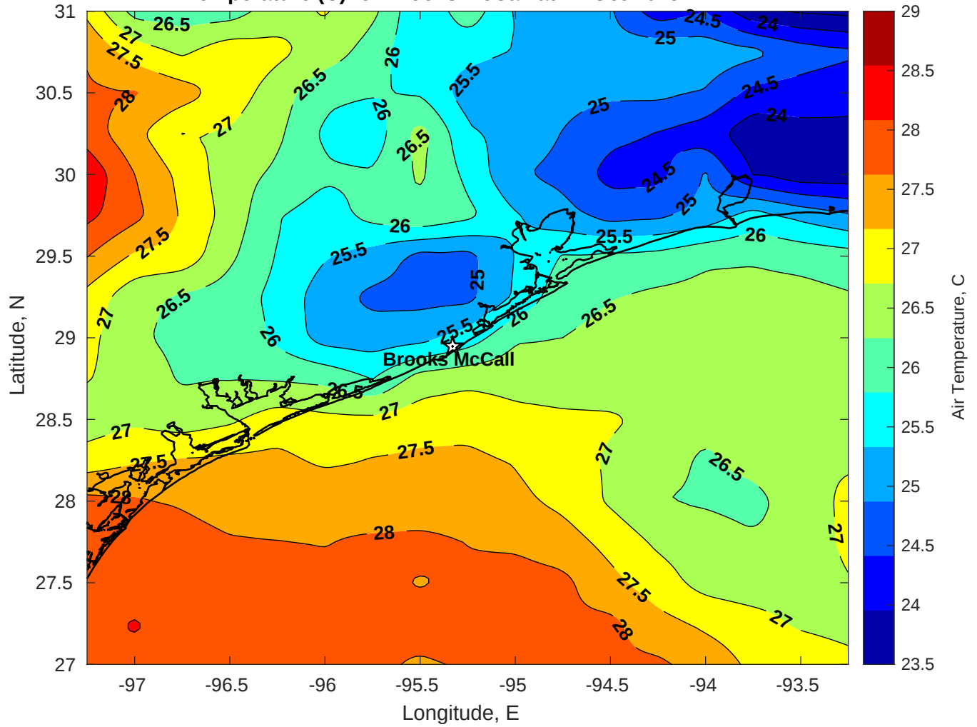
Air Temperature (C) for Brooks McCall at 24-Oct-2025
