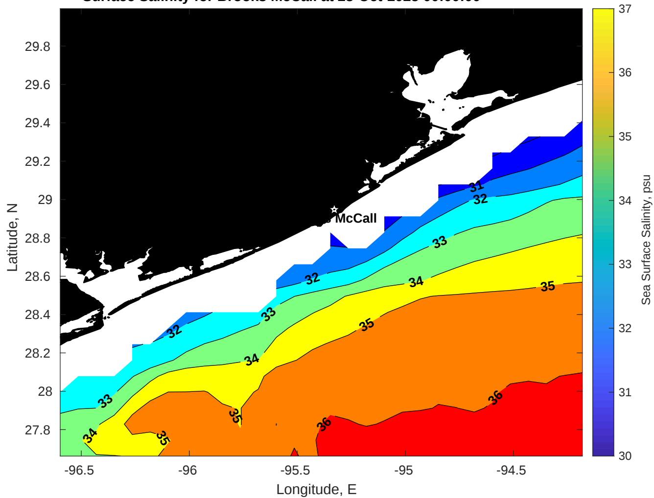
Surface Salinity for Brooks McCall at 23-Oct-2025 00:00:00
