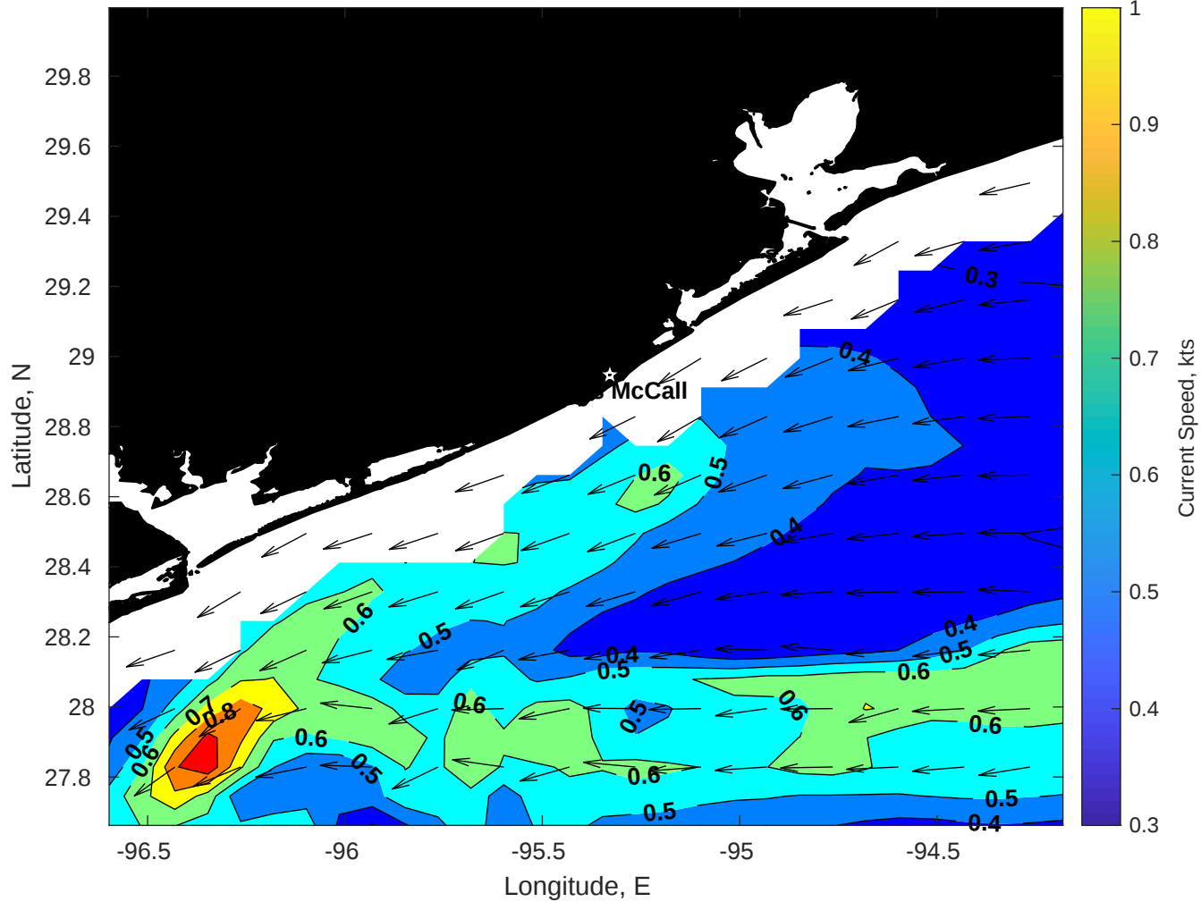
Surface Currents for Brooks McCall at 23-Oct-2025 00:00:00
