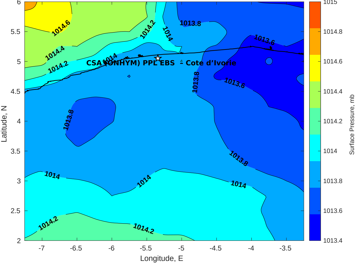
Surface Pressure (mb) for CSA (ONHYM) PPL EBS - Cote d'Ivoire at 24-Oct-2025 00:00:00
