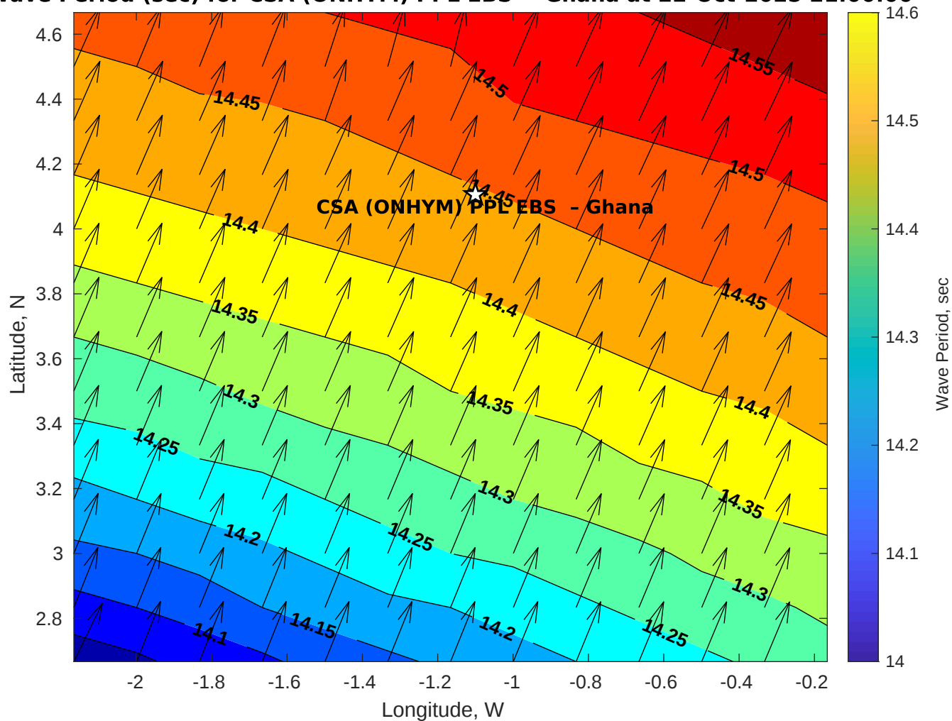
Wave Period (sec) for CSA (ONHYM) PPL EBS - Ghana at 22-Oct-2025 21:00:00
